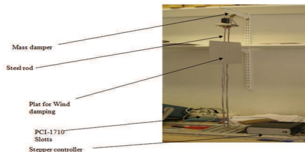
Fig. 7. Experimental Setup
