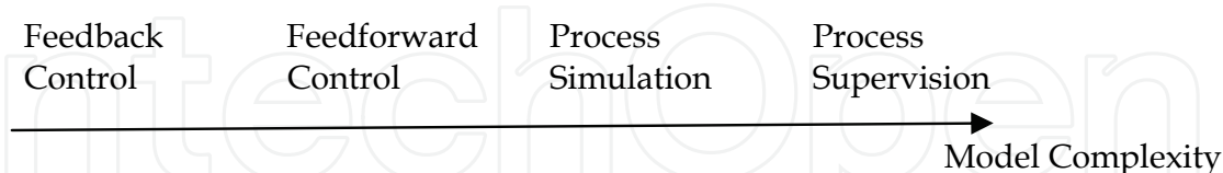
Fig. 1. Model Complexity
