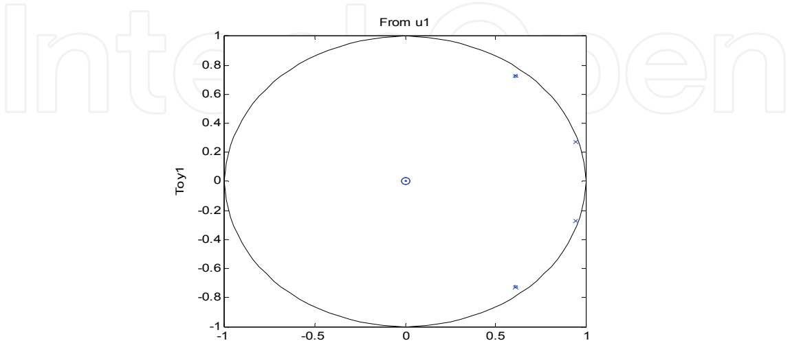
Figure 17: Pole-Zero Diagram
