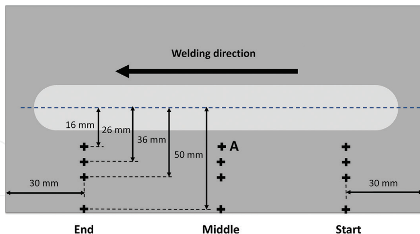
Figure 7. Location scheme of experimental measured points.
