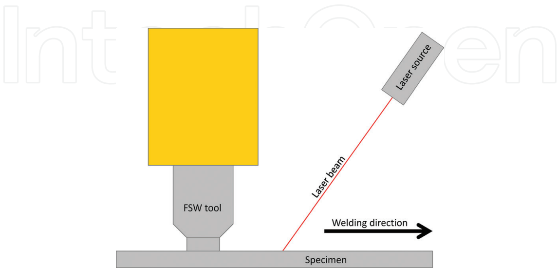
Figure 3. Scheme of the LAFSW setup.
