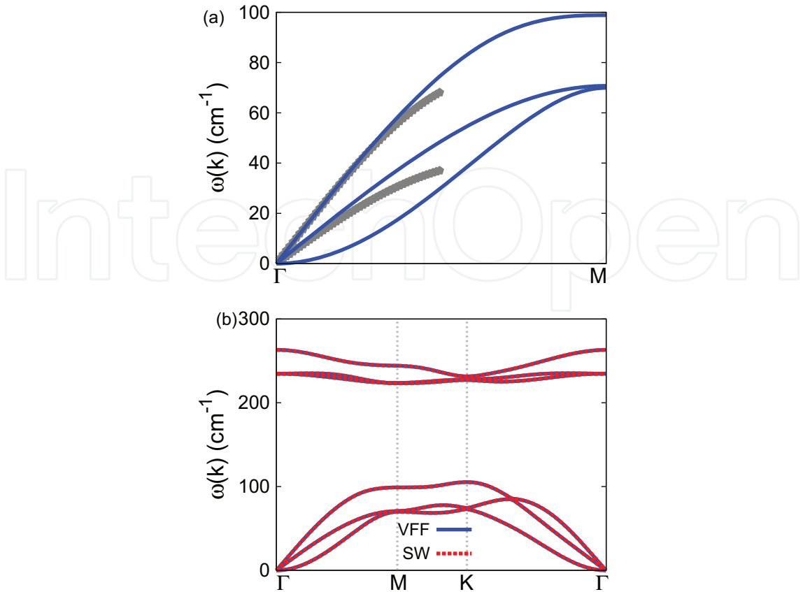
Figure 262. Phonon dispersion for the single-layer b-GeTe. (a) The VFF model is fitted to the two in-plane acoustic branches in the long wave limit along the \Gamma M direction. The ab initio results (gray pentagons) are calculated from SIESTA. (b) The VFF model (blue lines) and the SW potential (red lines) give the same phonon dispersion for the b-GeTe along \Gamma MK \Gamma .
