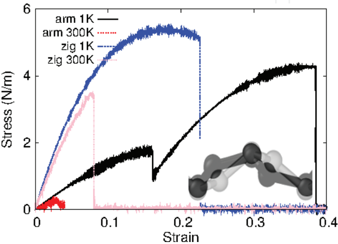
Figure 199. Stress-strain relations for the single-layer p-CS of size 100 × 100 Å. The single-layer p-CS is uniaxially stretched along the armchair or zigzag directions at temperatures 1 and 300 K. Inset shows the structure before (light) and after (dark) the structural transition around 0.16.
