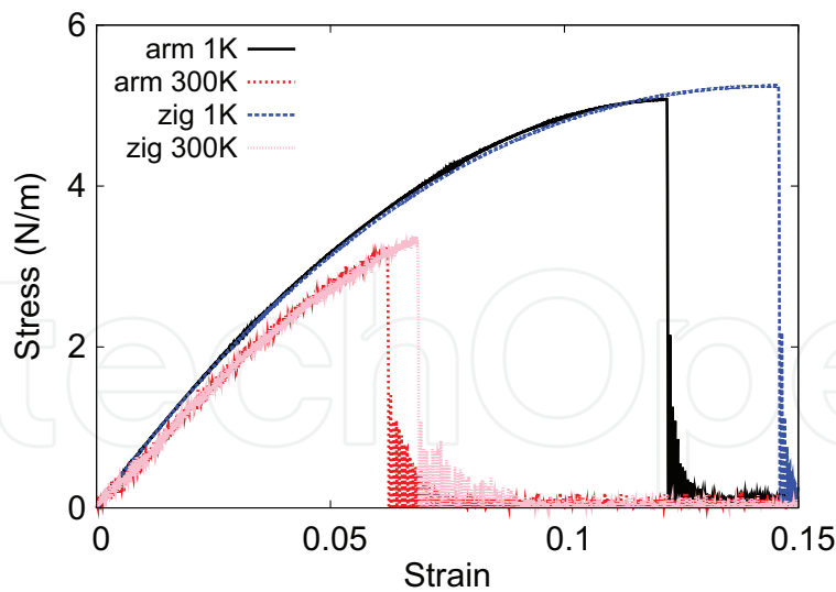
Figure 162. Stress-strain for single-layer 1T-WTe 2 of dimension 100 \times 100 Å along the armchair and zigzag directions.
