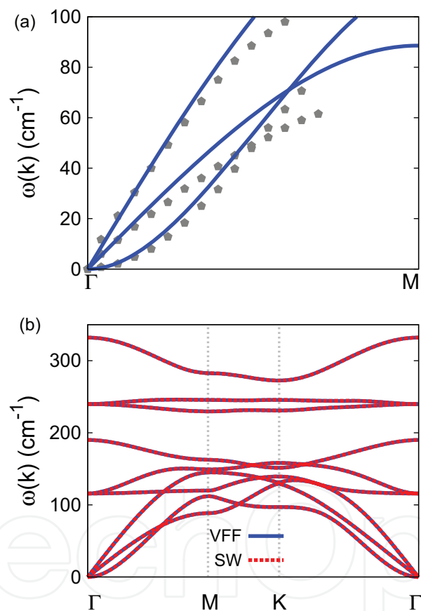
Figure 57. Phonon dispersion for single-layer 1H-MoTe 2 . (a) The VFF model is fitted to the three acoustic branches in the long wave limit along the \Gamma\text{M} direction. The ab initio results (gray pentagons) are from Ref. [36]. (b) The VFF model (blue lines) and the SW potential (red lines) give the same phonon dispersion for single-layer 1H-MoTe 2 along \Gamma\text{MK}\Gamma .
