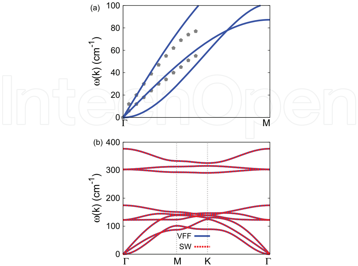
Figure 37. Phonon spectrum for single-layer 1H-FeTe 2 . (a) Phonon dispersion along the \Gamma M direction in the Brillouin zone. The results from the VFF model (lines) are comparable with the ab initio results (pentagons) from Ref. [12]. (b) The phonon dispersion from the SW potential is exactly the same as that from the VFF model.
