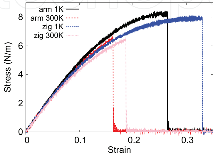
Figure 40. Stress-strain for single-layer 1H-CoTe 2 of dimension 100 × 100 Å along the armchair and zigzag directions.
