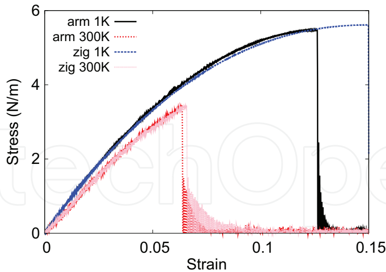
Figure 160. Stress-strain for single-layer 1T-WSe 2 of dimension 100 × 100 Å along the armchair and zigzag directions.
