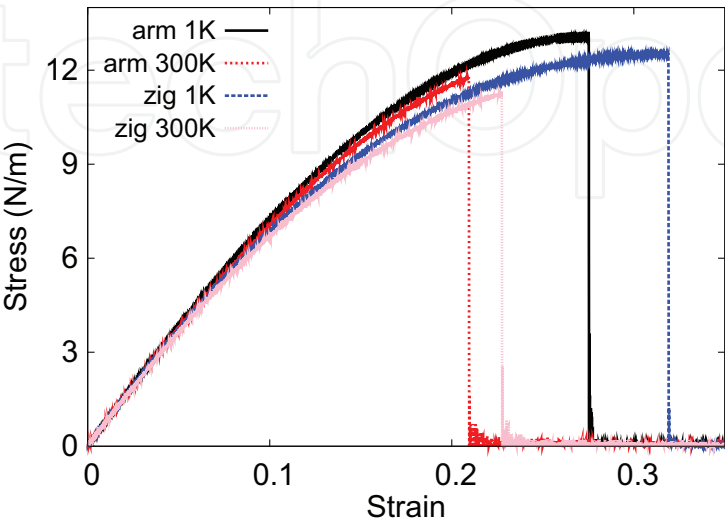
Figure 89. Stress-strain for single-layer 1T-VSe 2 of dimension 100 × 100 Å along the armchair and zigzag directions.
