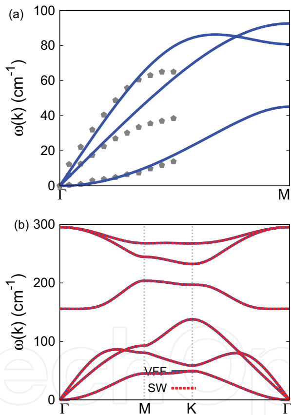
Figure 272. Phonon dispersion for the single-layer b-SnGe. (a) The VFF model is fitted to the three acoustic branches in the long wave limit along the \Gamma M direction. The ab initio results (gray pentagons) are from [114]. (b) The VFF model (blue lines) and the SW potential (red lines) give the same phonon dispersion for the b-SnGe along \Gamma MK \Gamma .
