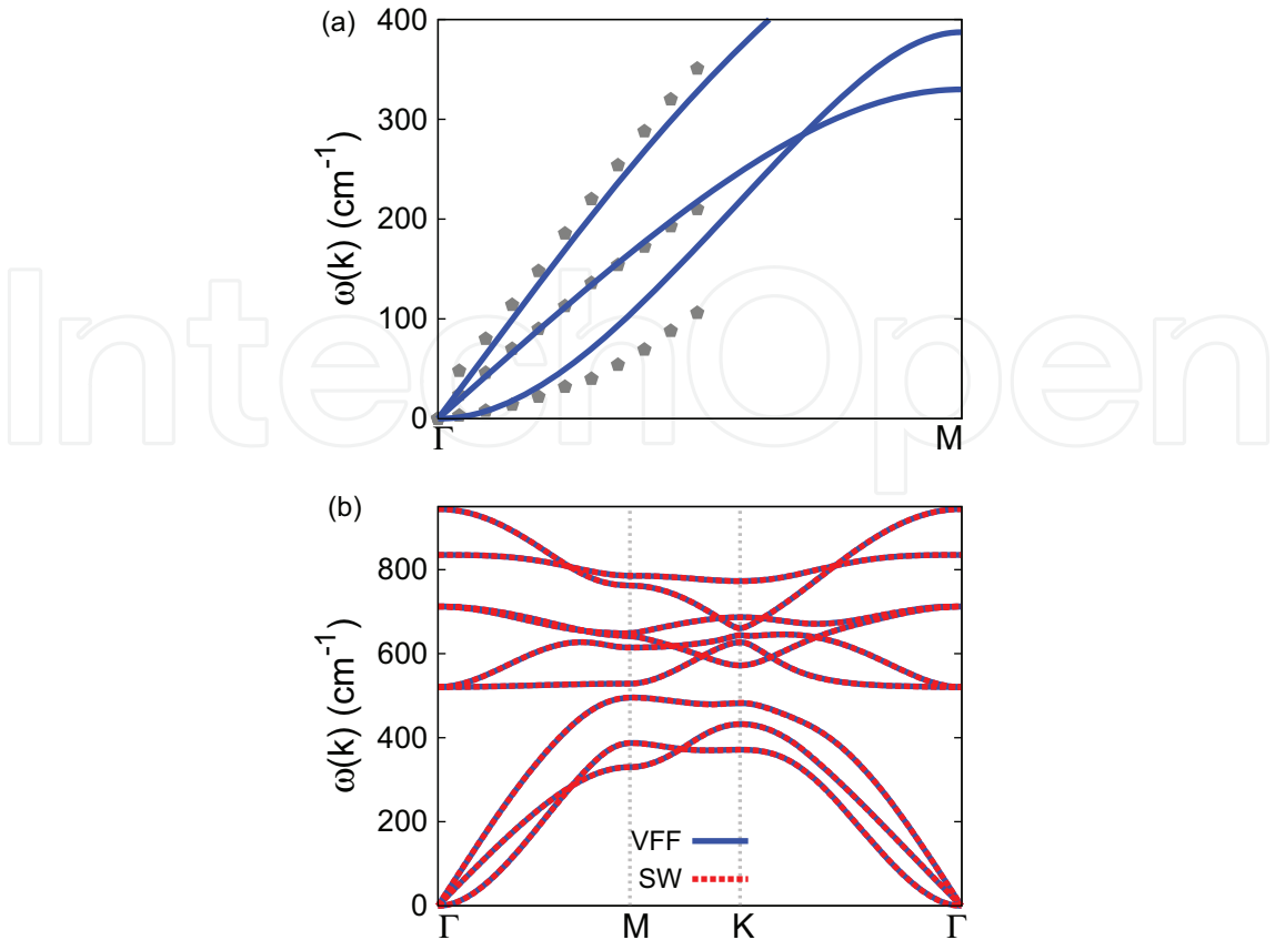
Figure 21. Phonon spectrum for single-layer 1H-CrO 2 . (a) Phonon dispersion along the \Gamma M direction in the Brillouin zone. The results from the VFF model (lines) are comparable with the ab initio results (pentagons) from [12]. (b) The phonon dispersion from the SW potential is exactly the same as that from the VFF model.
