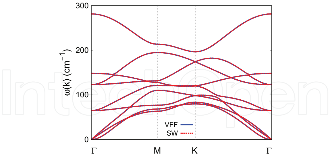
Figure 133. Phonon spectrum for single-layer 1T-TcTe 2 along the \Gamma MK \Gamma direction in the Brillouin zone. The phonon dispersion from the SW potential is exactly the same as that from the VFF model.
