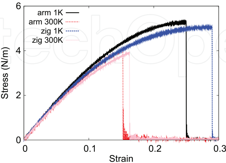
Figure 77. Stress-strain for single-layer 1T-ScSe 2 of dimension 100 × 100 Å along the armchair and zigzag directions.
