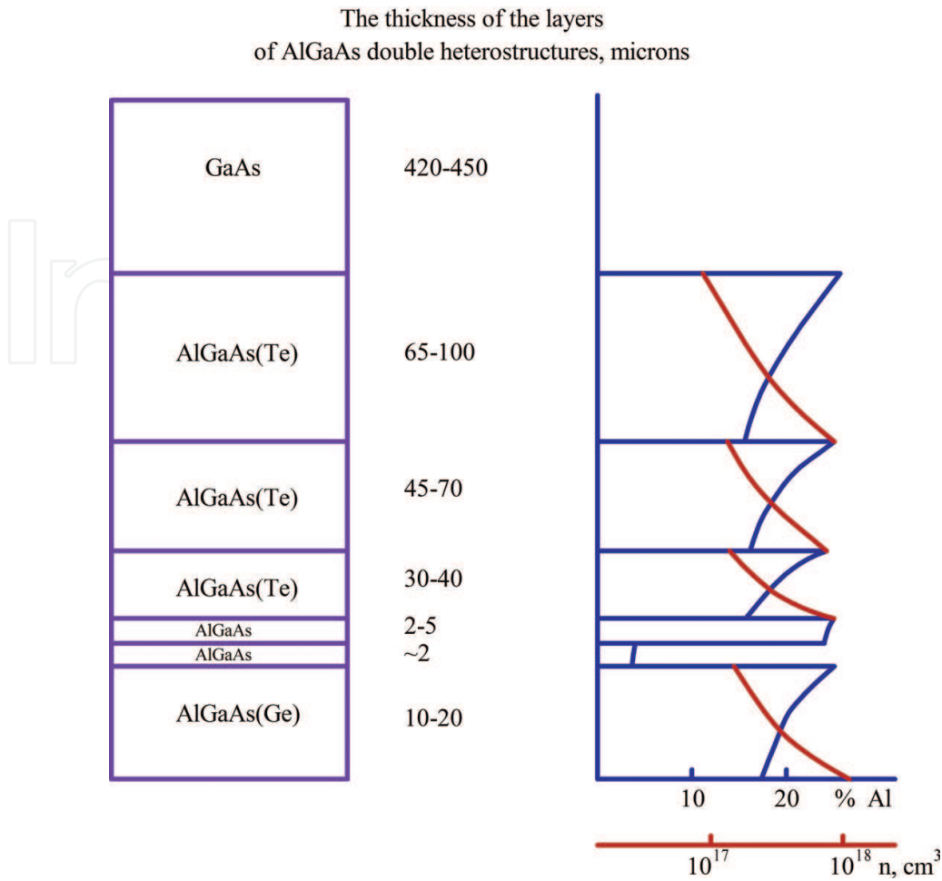
Figure 1. Structure of the double AlGaAs heterostructure.
