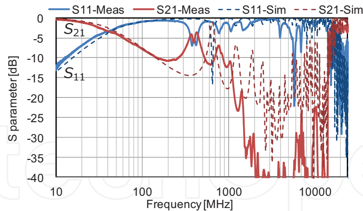
Figure 10. Measured results of DC waveguide.
