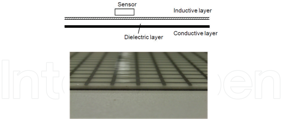
Figure 8. Sheet-type waveguide [52].
