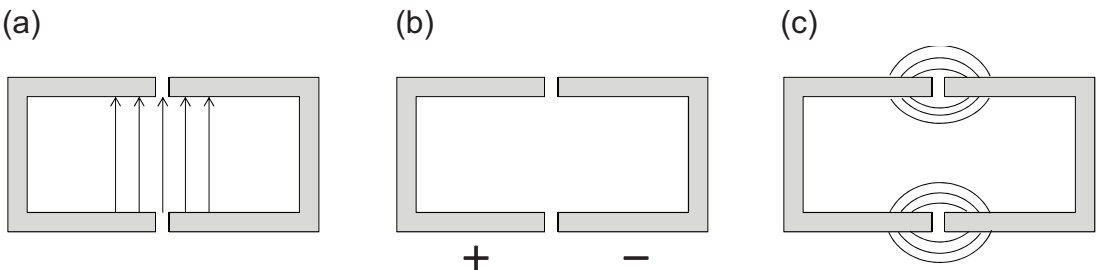
Figure 9. Propagation modes of the split waveguide.
