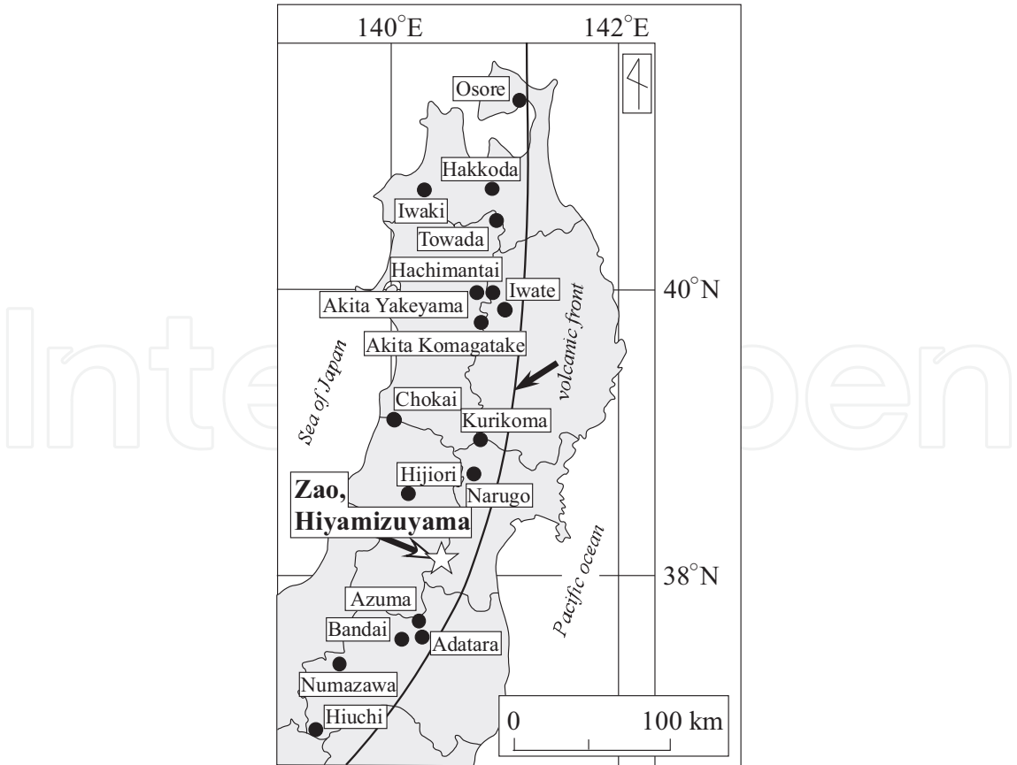
Figure 1. Locality map of Zao and Hiyamizuyama volcanoes. Eighteen active volcanoes, including Zao volcano, in NE Japan are plotted.
