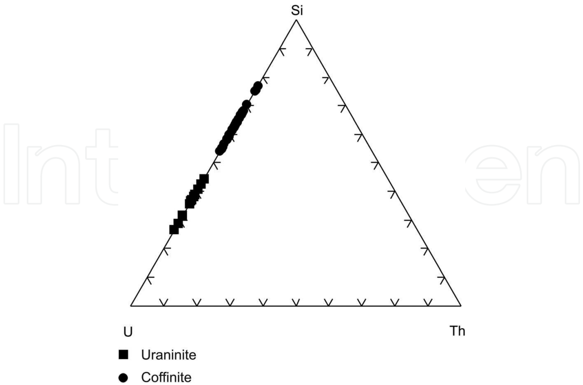
Figure 9. Chemical composition of coffinite and uraninite from the Rožná uranium deposit (wt.%).
