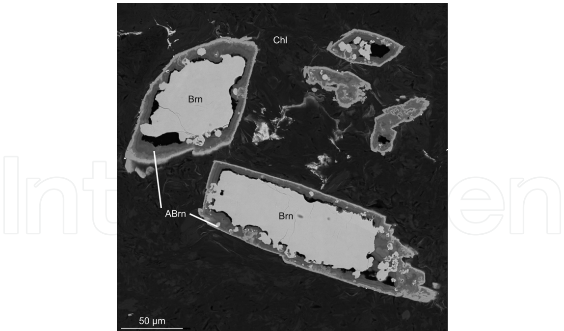
Figure 10. BSE image of brannerite (Brn) and altered brannerite (ABrn) enclosed in finely grained chlorite (Chl) from the Zadní Chodov uranium deposit.
