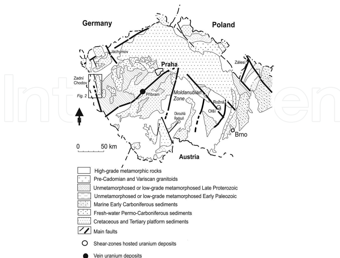
Figure 1. Simplified geological map of the Bohemian Massif with the most significant hydrothermal uranium deposits.
