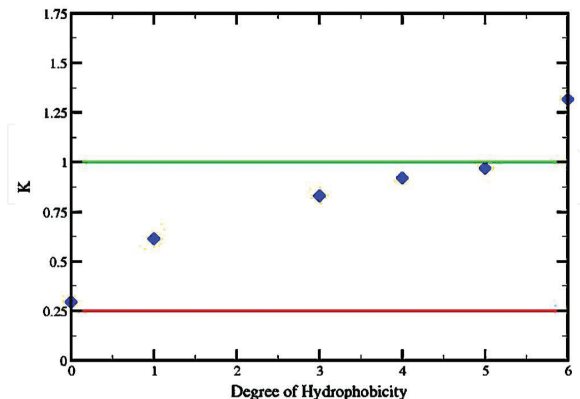
Figure 12. Normalized variance as the function of degree of hydrophobicity.
