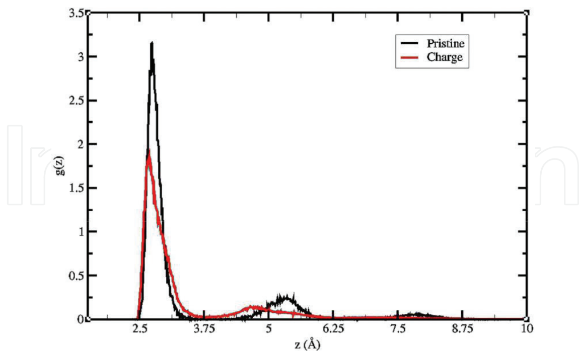
Figure 8. Decrease in the ordering of confined water inside CNT.
