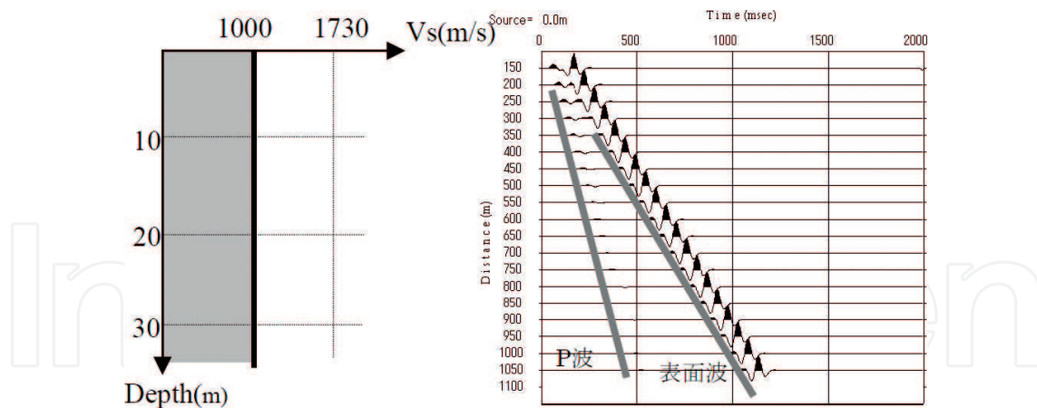
Figure 5. A soil model with velocity of 1000 m/s [4].
