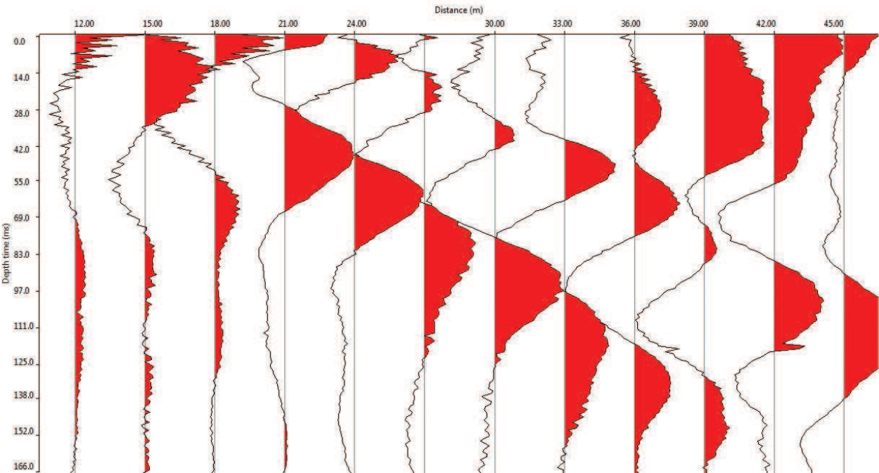
Figure 15. The record of field shot gather.
