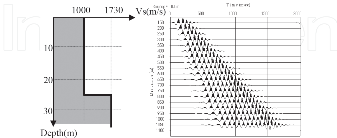
Figure 7. Combination of soil model with velocity of 1000 m/s and of 1730 m/s [4].
