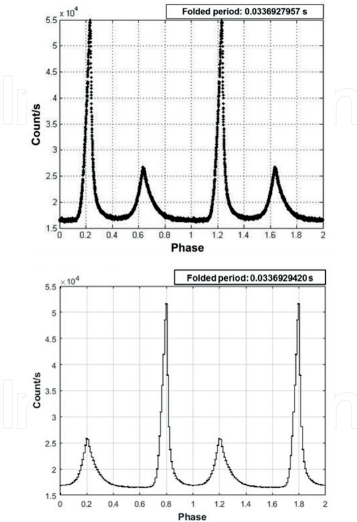
Figure 6. Top: Crab pulsar light curve obtained from data collected with SiFAP by using the Fourier approach. Bottom: Crab pulsar light curve obtained from data collected with SiFAP by using the EFS approach. The phase shift is due to the slight difference between the two computed spin periods.
