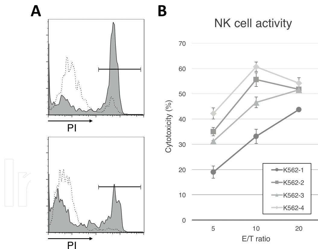
Figure 1. Variation in the results of assaying for NK activity due to differences in the pre-culture conditions of target cells. K562 cells were pre-cultured under four different conditions using two different cell densities prepared separately by two individuals. A shows representative histograms of K562 cells obtained by flow cytometry with a high percentage of PI + dead cells (upper) and low percentage of cells (lower) at an E/T ratio of 10 following incubation with human PBMCs for 4 h. K562 cells were distinguished from PBMCs by positive DiO staining and gated to show the histograms. The bar represents the region defined and measured as the population of DiO + PI + cells. Dashed lines represent targets alone. A summarized graph with mean and SD from the three wells is shown in B. It is clear that the cytotoxicity obtained from the assay with K562-1 shows only half the degree of cytotoxicity obtained from the assay with K562-4.
