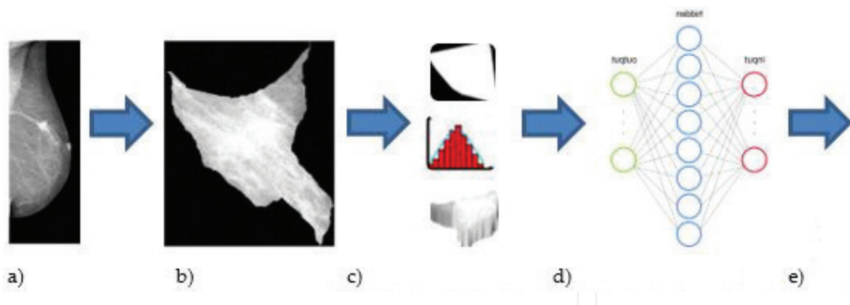
Figure 8. Training of GRANN for BCD. (a) Breast image, (b) segmentation, (c) image descriptors, (d) network training, and (e) BCD.
