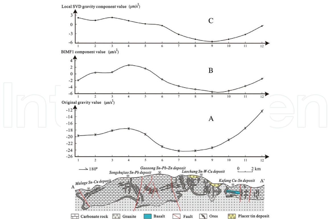
Figure 6. Spatial relationships between granites, ore bodies and local gravity components cross the section AA' in the Gejiu tin-copper polymetallic ore field shown in Figure 5 (modified from [10, 11]). (A) Original gravity anomaly; (B) the BIMF 1 gravity component decomposed from the original gravity anomaly by using BEMD; (C) local gravity component decomposed from the original gravity anomaly by using SVD [13].
