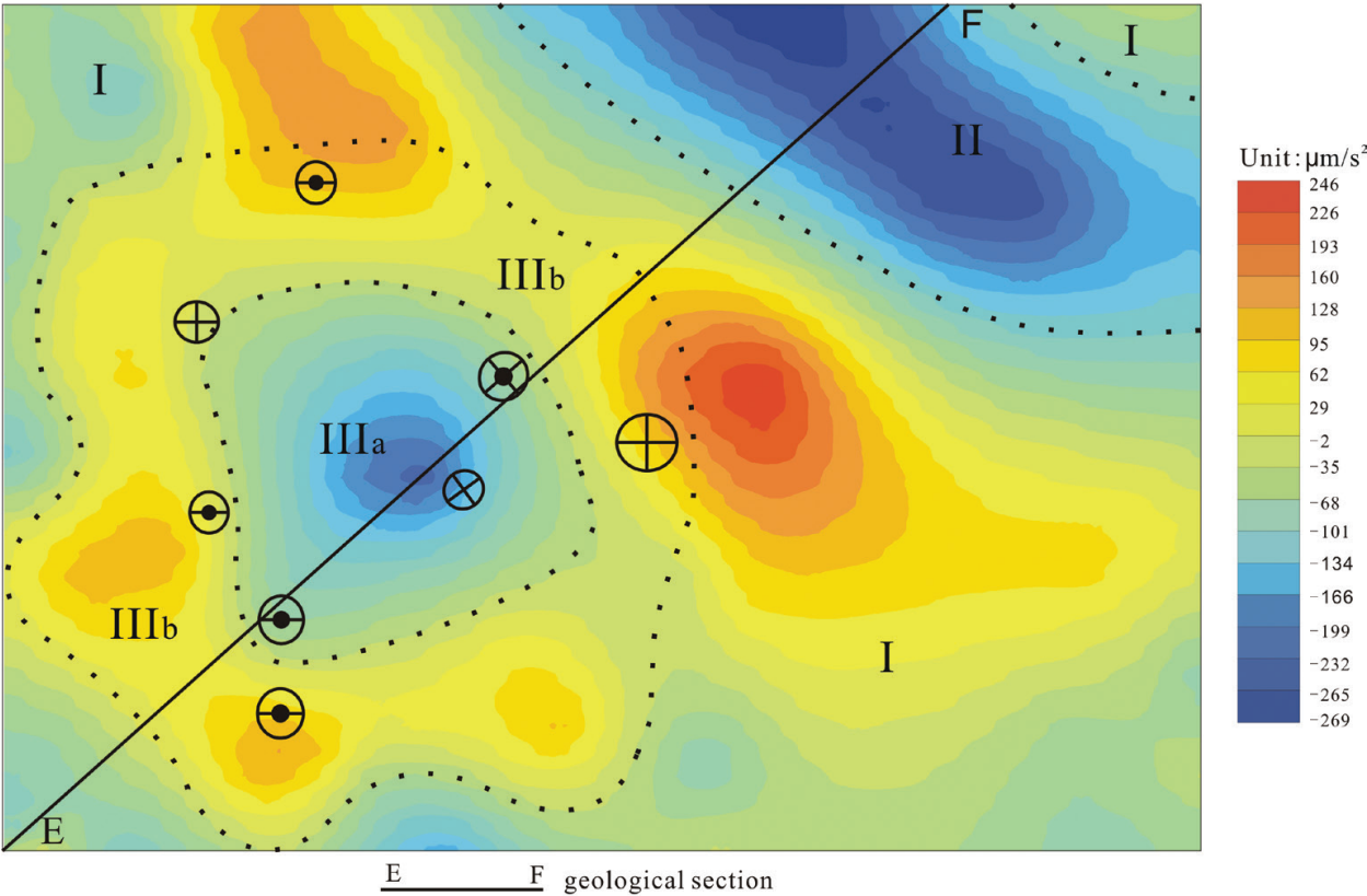
Unit I: concealed basement; Unit II: Mesozoic volcanic sedimentary basin; Unit IIIa: Tongshi intrusive complex; Unit IIIb: contact metasomatic zone between the Tongshi intrusive complex and its host rocks
