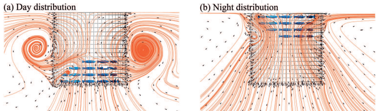
Figure 11. The flow around fish cage for different distributions in still water with 0.45 BL/s fish speed (a, b).
