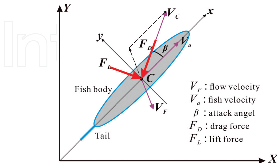
Figure 4. Top view of the tail-actuated fish model.
