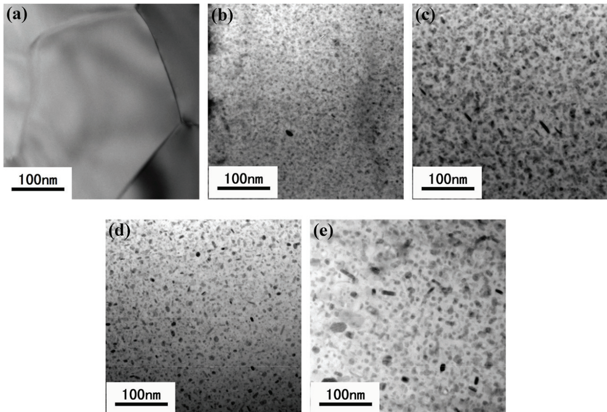
Figure 4. TEM images of MPts of AA7050 with different initial tempers before creep aging tests: (a) solution; (b) T6; (c) T73; (d) retrogression; (e) re-solution.
