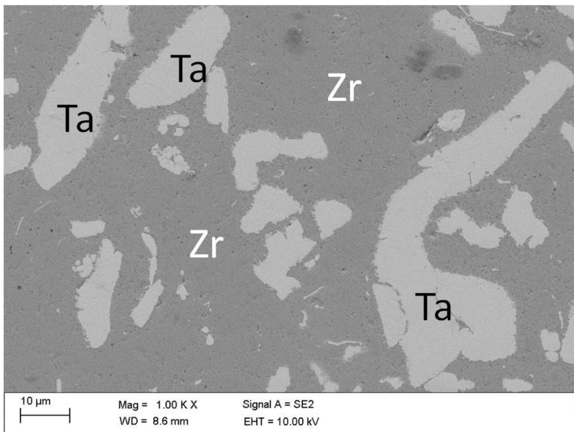
Figure 2. FE-SEM image of the \text{ZrO}_2\text{:Ta} cermet used for performing experiments.
