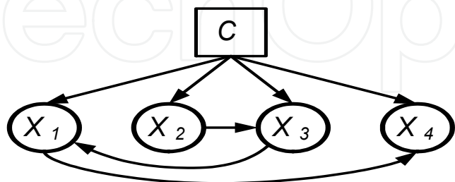
Fig. 2. Example of a Tree-Augmented bayesian Network (TAN)
