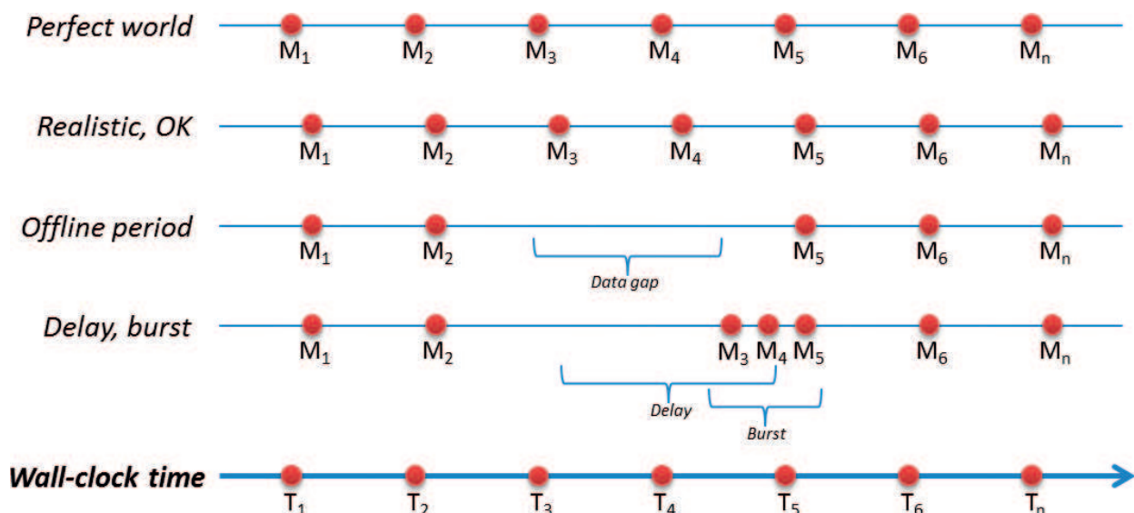
Figure 2. Aspects of timeliness. The display dots (M1-Mn) represent input data created at wall clock time T1-Tn.
