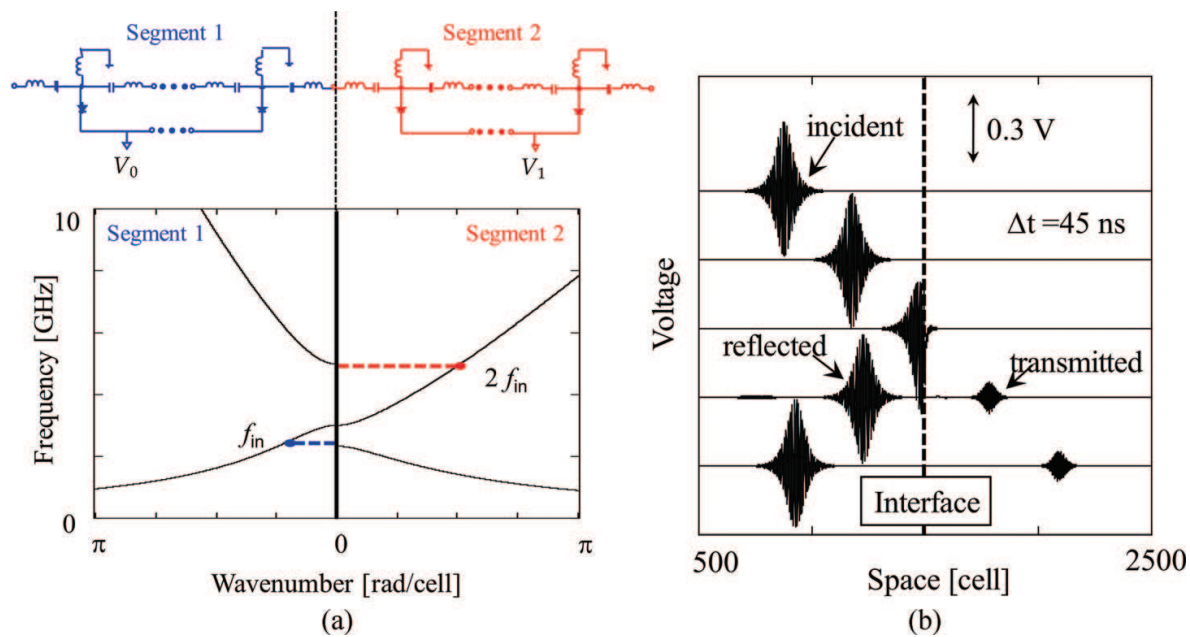
Figure 4. Effective method of second harmonic generation. (a) The device structure (upper), dispersive property of each segment (lower), and (b) the numerically obtained time-domain waveforms.
