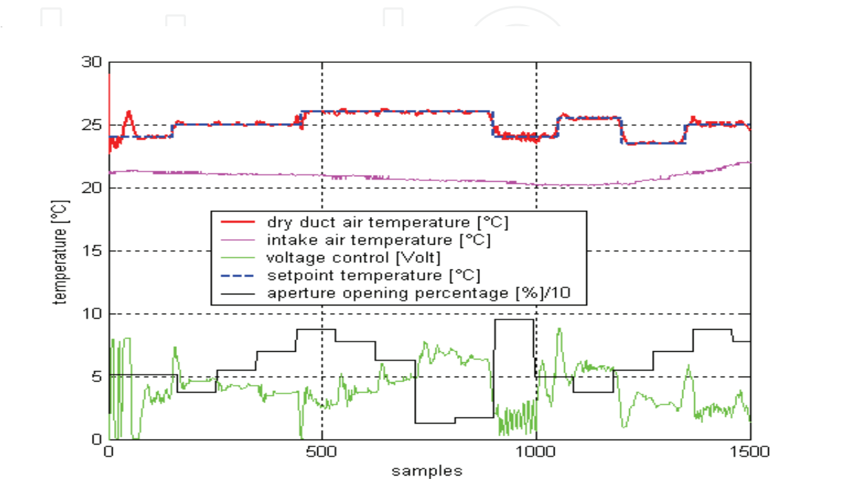
Fig. 4. IAGPC of the air dry duct temperature
