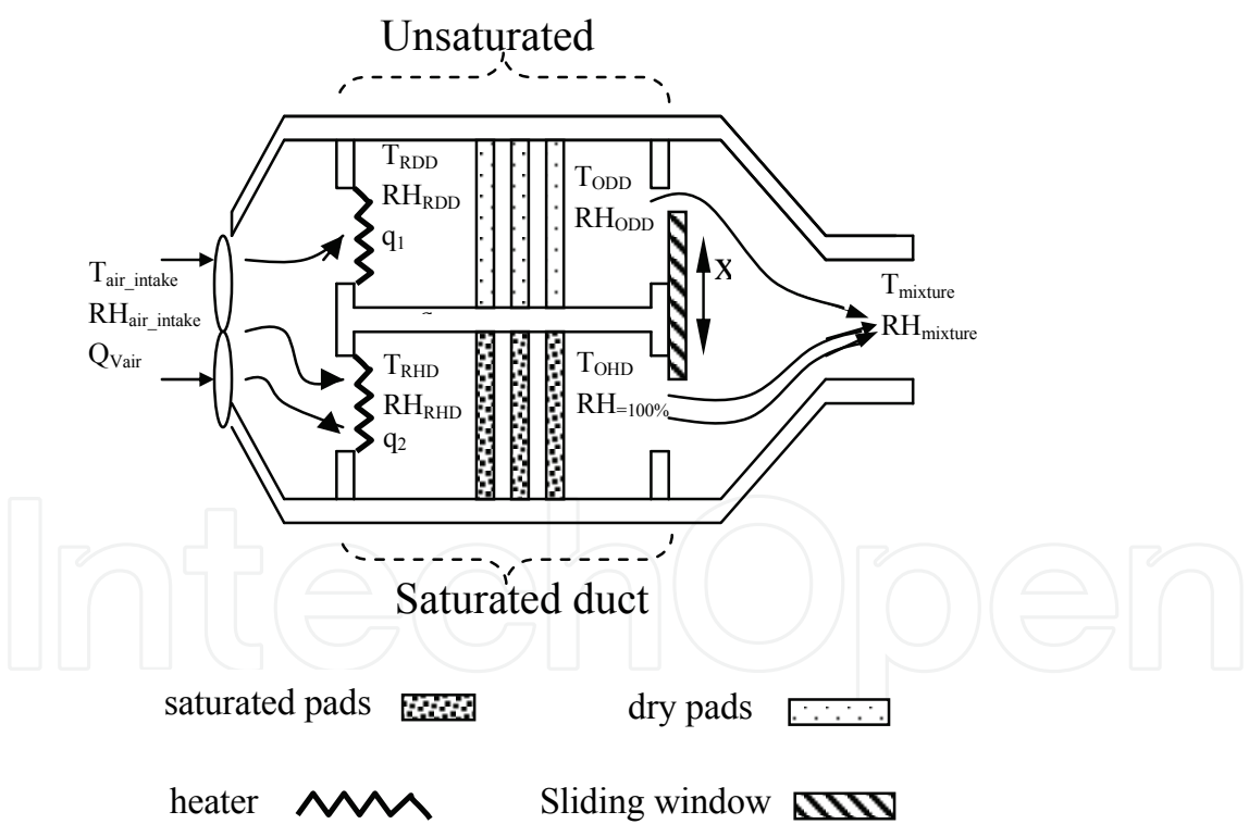
Fig. 2. Air-conditioning system
