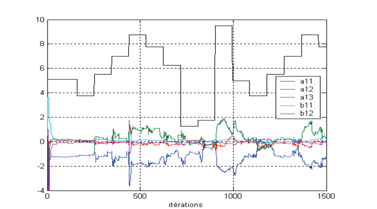
Fig. 5. Dry duct model estimated parameters
