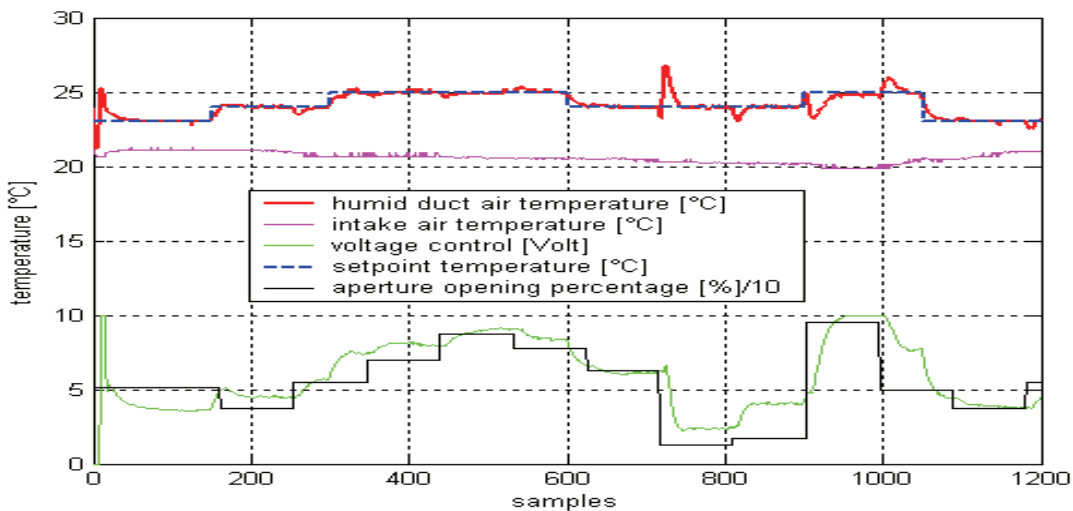
Fig. 10. DAGPC of the air humid duct temperature
