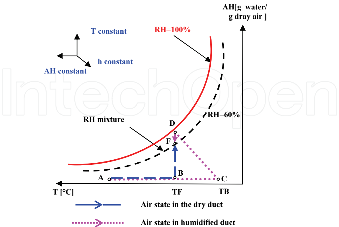
Fig. 1. Thermodynamic cycle of the unit
