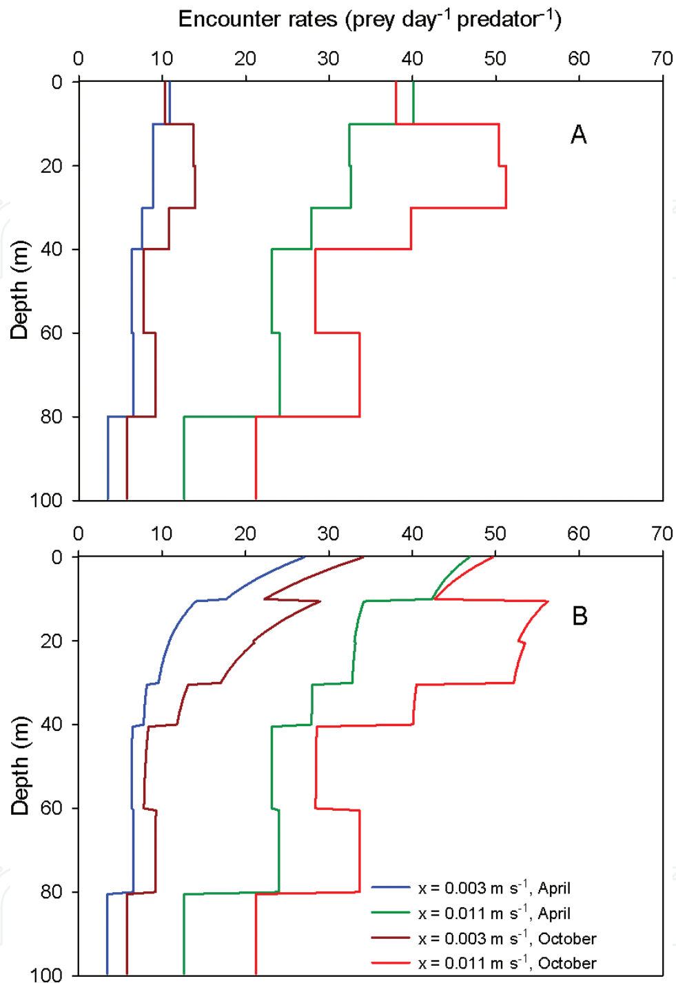
Figure 2. Encounter rates between siphonophores and fish larvae under non-turbulent (A) and turbulent (B) conditions in the southern Gulf of Mexico.
