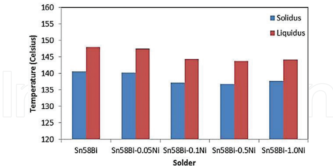
Figure 12. Solidus and liquidus temperatures of Sn–58Bi–xNi [29].
