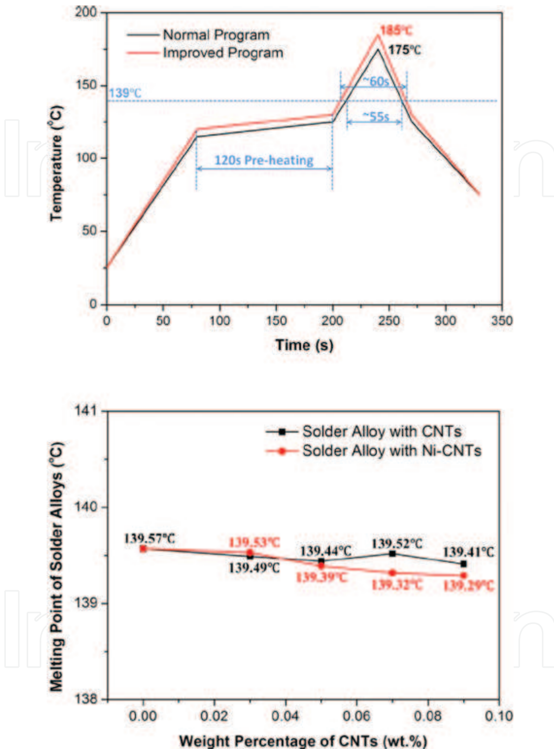
Figure 15. Plot of the variation of melting point of solder alloys with different amounts of CNTs or NI-CNTs [35].
