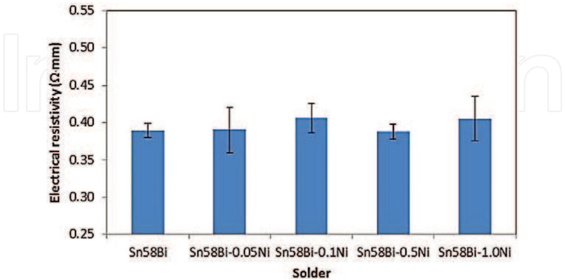
Figure 10. Electrical resistivity of Sn-58Bi-xNi [29].
