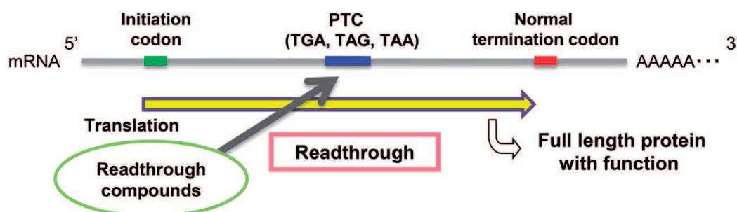
Figure 4. Nonsense mutation as a premature termination codon (PTC) and readthrough compounds. (A) mRNAs containing no PTC are translated into full-length and functional proteins. (B) In the case of mRNAs containing PTC, translation stops at PTC and non-functional truncated proteins are synthesized. (C) In the presence of readthrough compounds, even mRNAs containing PTC are translated into full-length and functional proteins.
