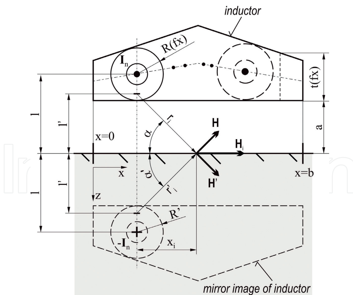
Figure 2. Inductor with a central peak.
