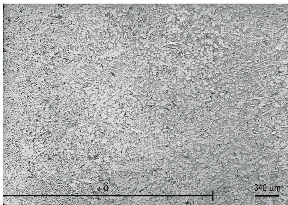
Figure 6. Microstructure of the AlSi8.5Cu alloy from the sample's edge to a distance of \delta .
