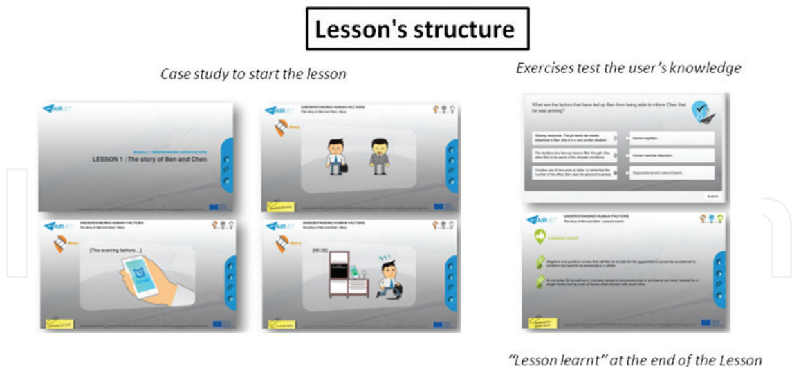
Figure 15. Lesson's structure.
