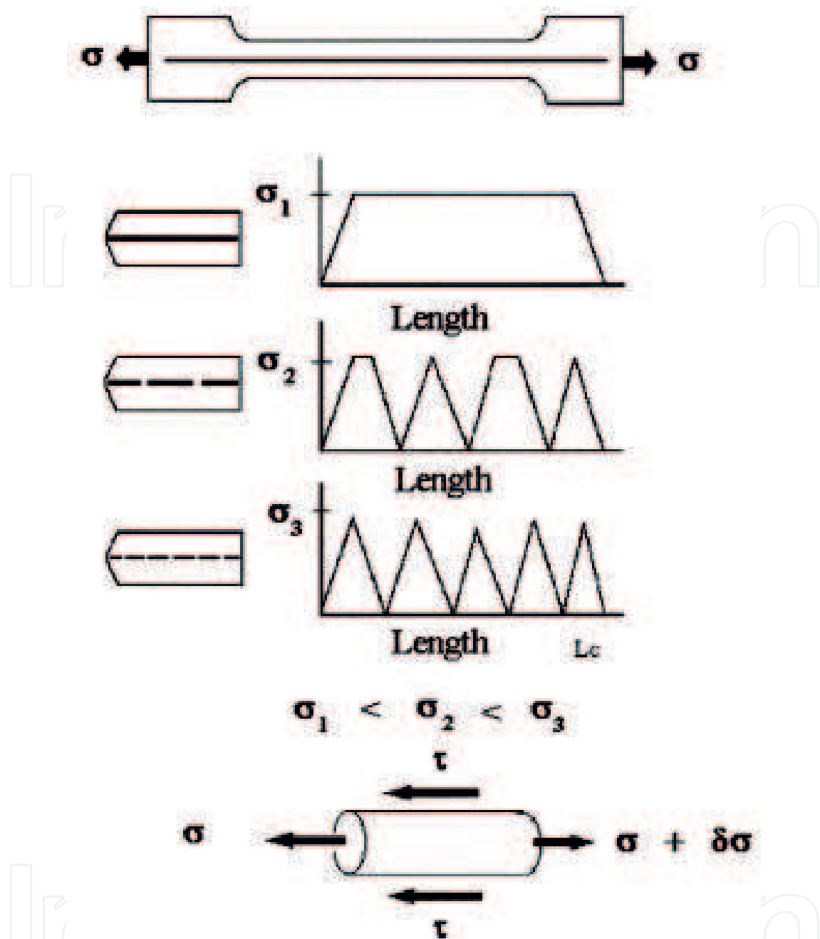
Figure 7. Schematic representation of the full fragmentation test [34].
