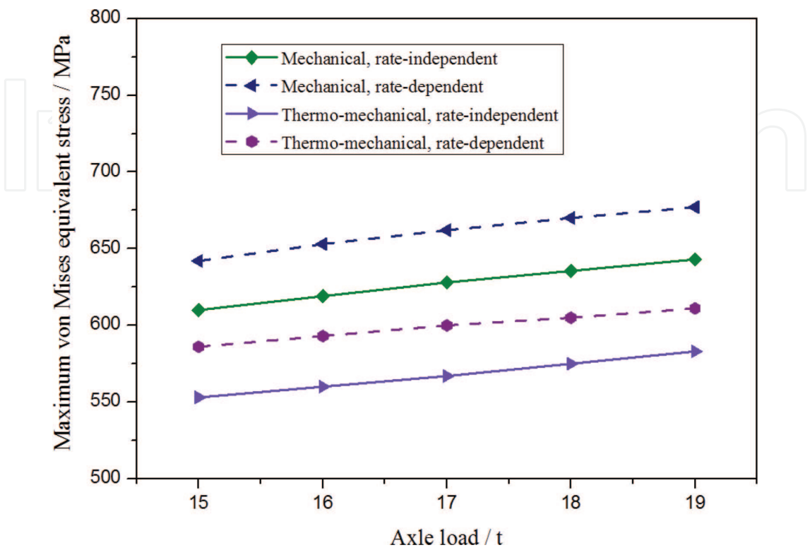
Figure 17. Maximum von Mises equivalent stresses as a function of axle load.
