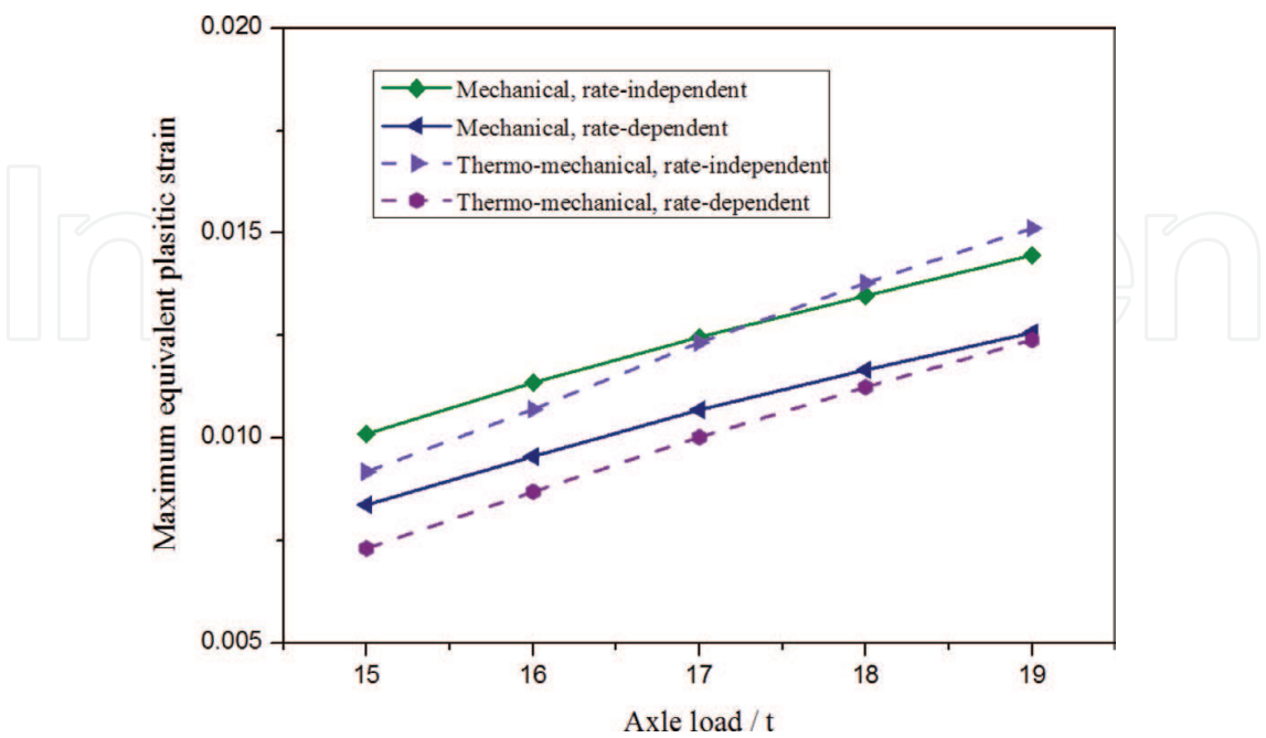
Figure 18. Maximum equivalent plastic strains as a function of axle load.
