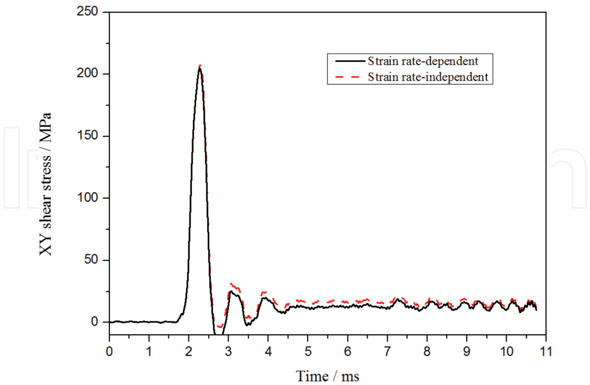
Figure 7. XY shear stress versus time curves (17t axle load, 200 km/h train speed and 40 mm flat).
