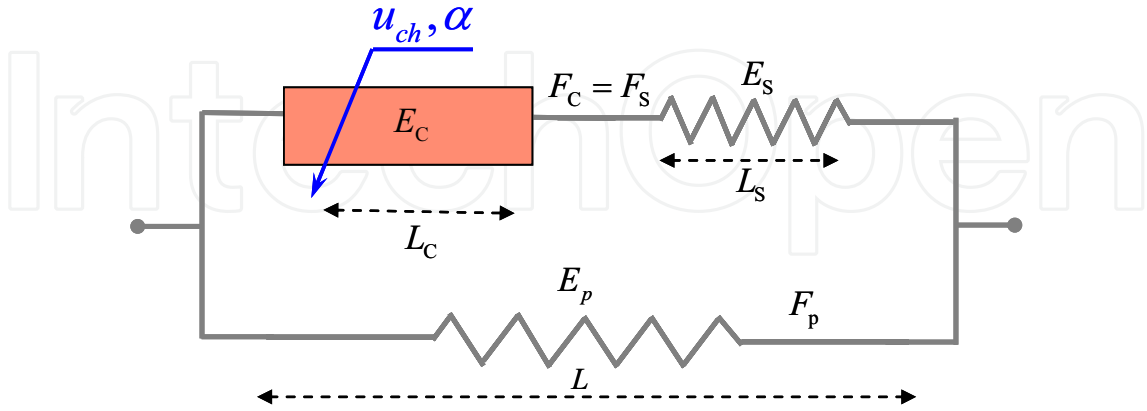
Fig. 3. Muscle model and particularity of E_c (El-Makssoud et al., 2004-a).
