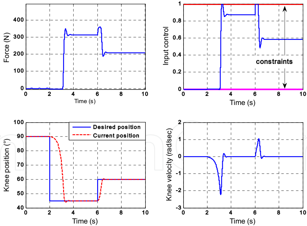
Fig. 12. Tracking knee joint trajectory and controller performance.
