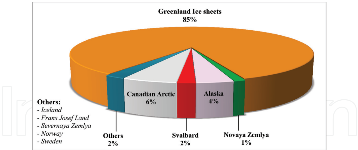
Figure 5. Percent contribution of 10 Arctic regions covered by extensive glaciation [4].
