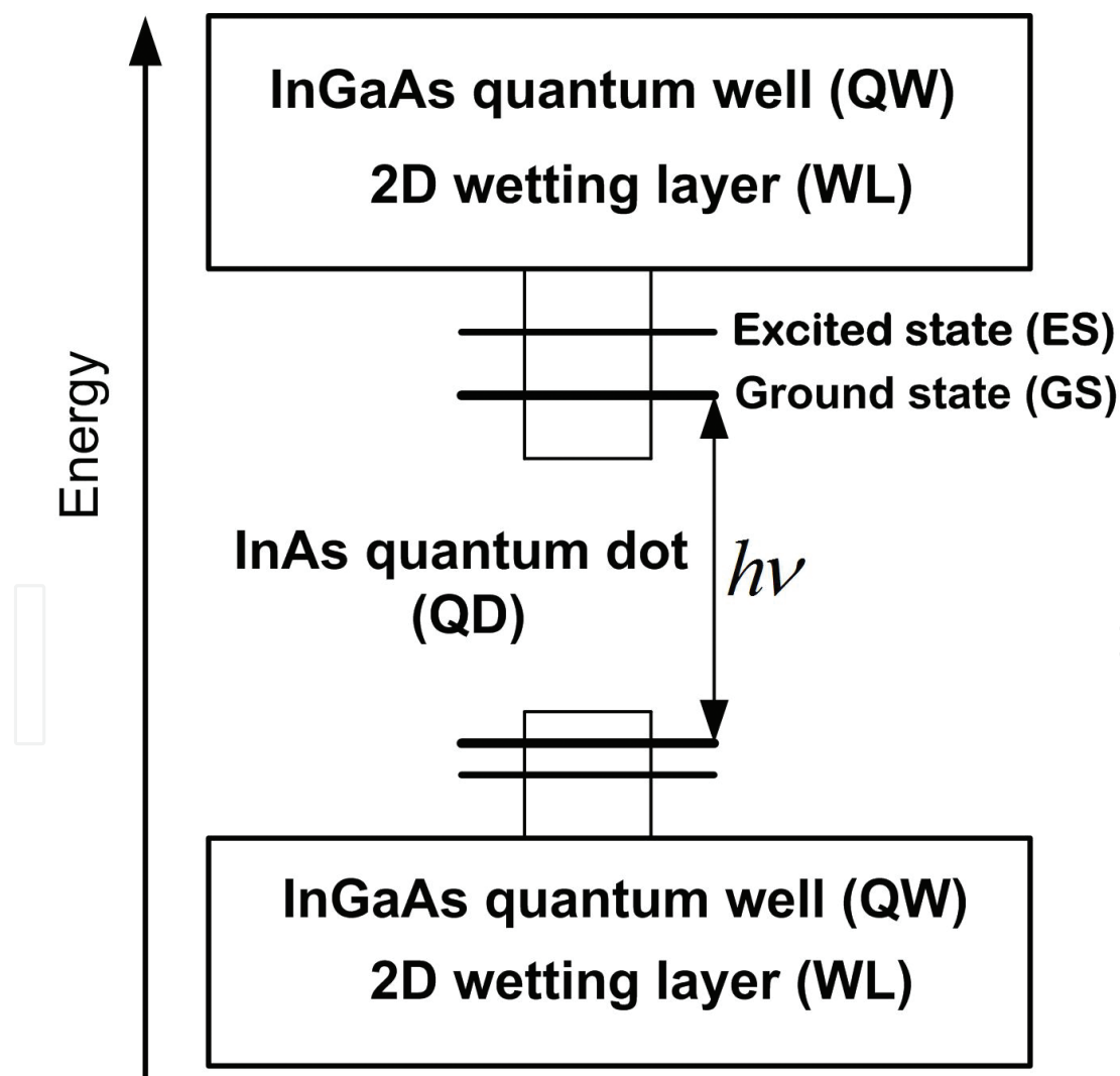
Figure 4. The energy band structure of a QDWELL laser.
