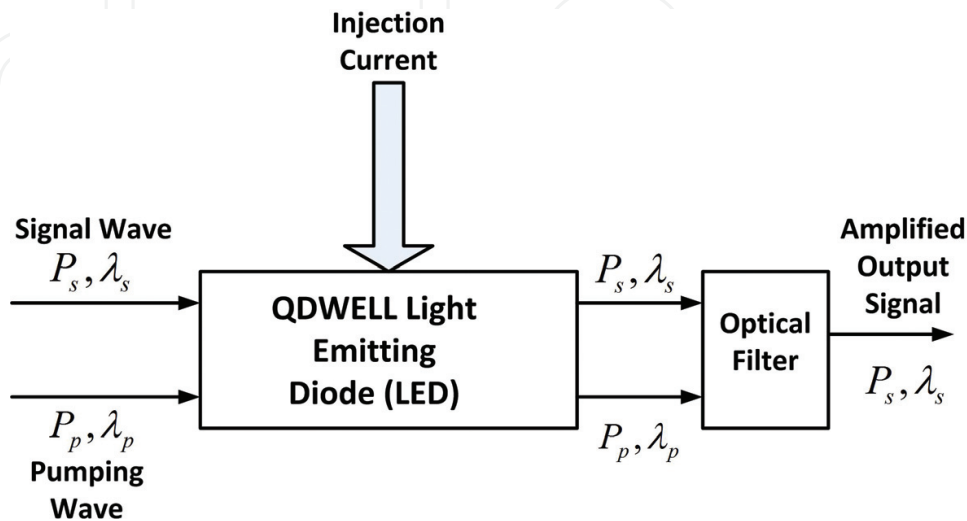
Figure 6. The block diagram of TWA QDWELL SOA.
