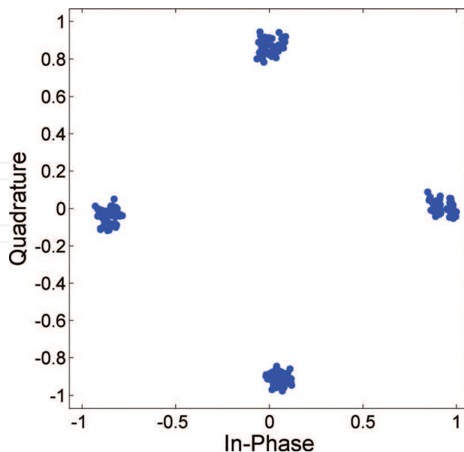
Figure 8. The calculated constellation of the output 4-QAM modulation signal for the modulation frequency 60 GHz, zero detuning, and the optical injection power of 1 mW.
