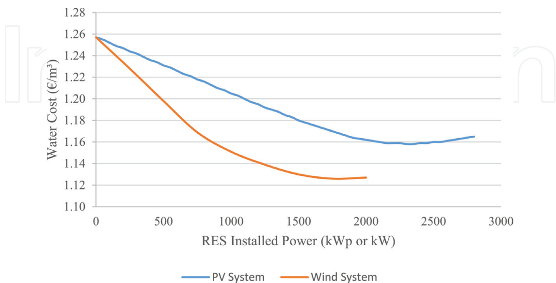
Figure 14. Water cost versus wind and photovoltaic install power for Hermoupolis. One technology each time.
