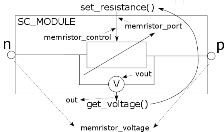
Figure 1. Block diagram for the selected SystemC-AMS model for a memristor.
