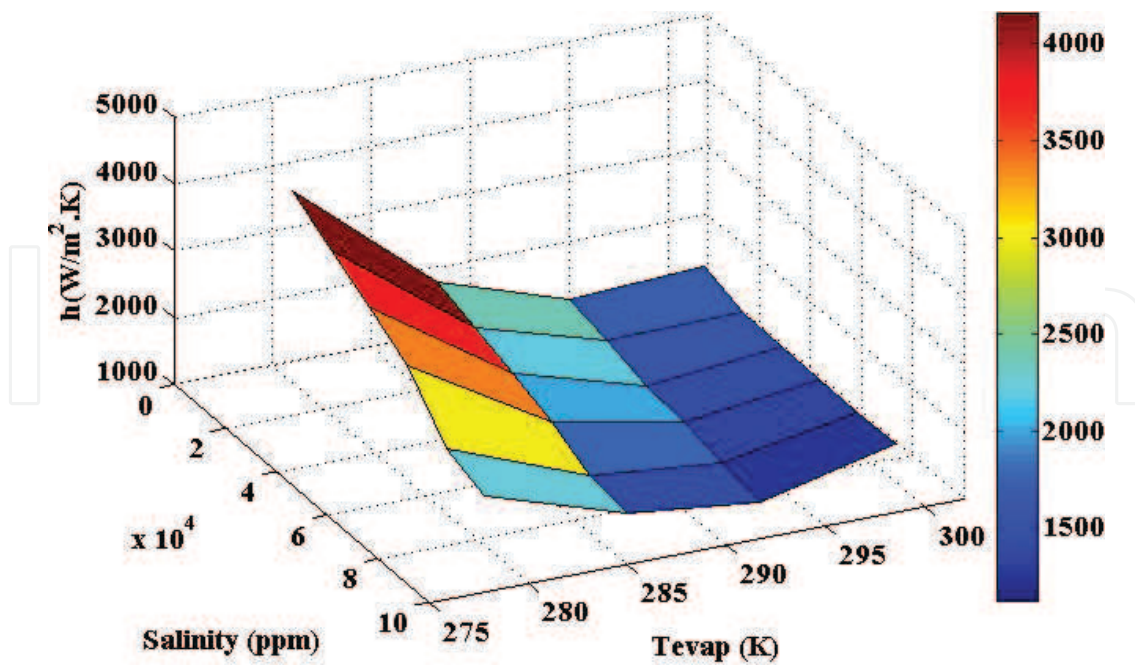
Figure 9. Experimental film evaporation heat transfer coefficient profiles at different saturation temperature and different salt concentrations.
