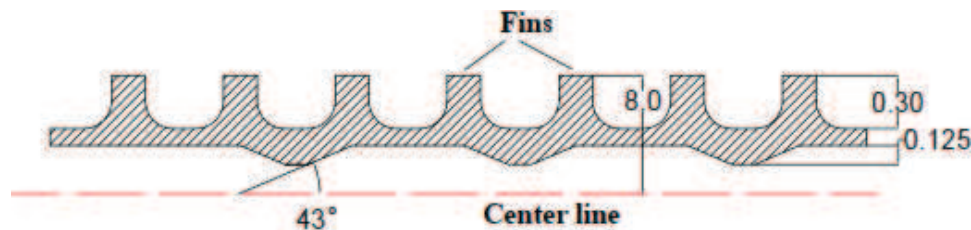
Figure 4. Cross section of end-cross tube used in evaporator of adsorption desalination plant.
