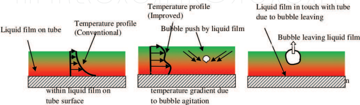
Figure 6. Film agitations due to bubbles movement and effect on conventional thermal gradient.
