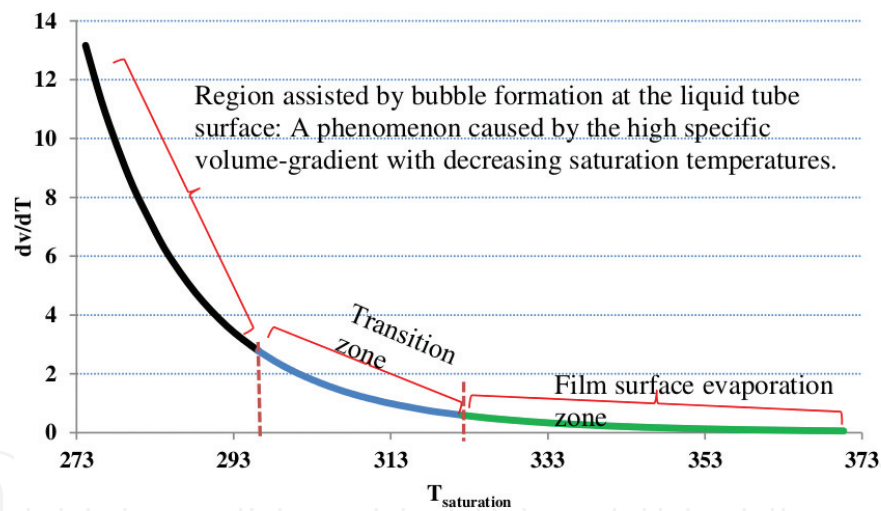
Figure 10. Change in vapour-specific volume with saturation temperature.
