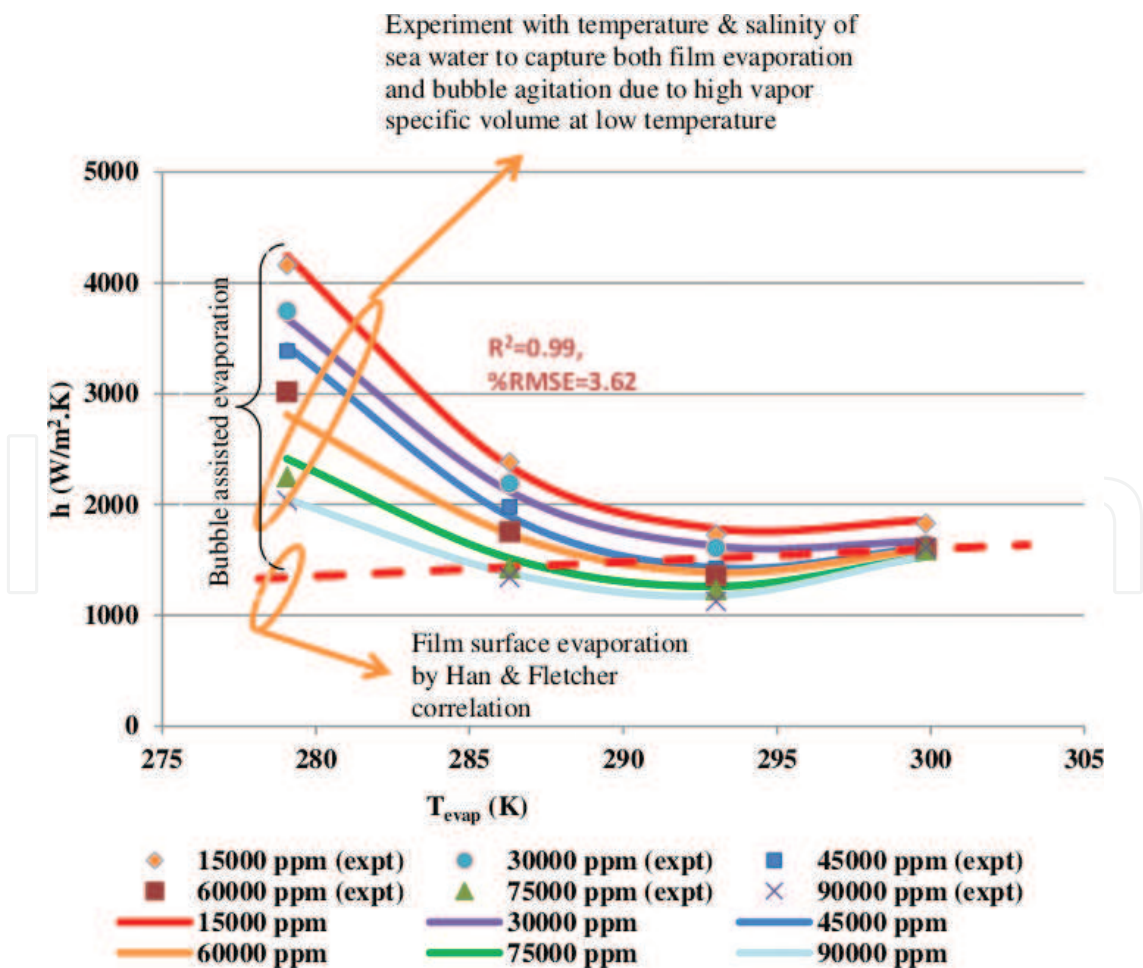
Figure 11. Falling film heat transfer coefficients values: experimental and proposed correlation.
