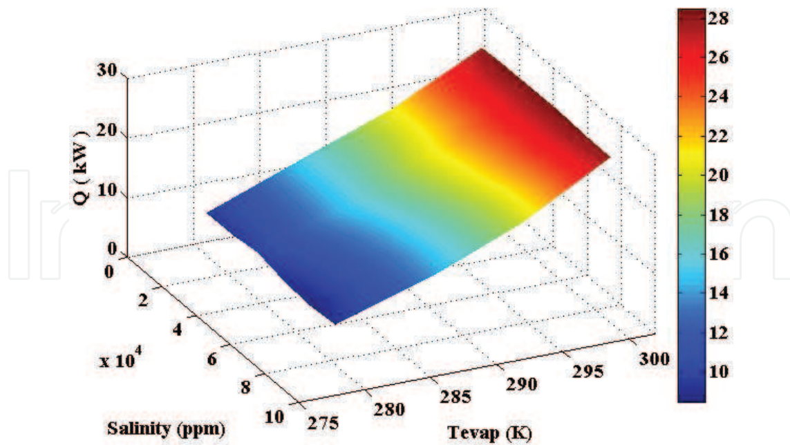
Figure 13. Effect of evaporator saturation temperature and feed salt concentration on heat input to evaporator.
