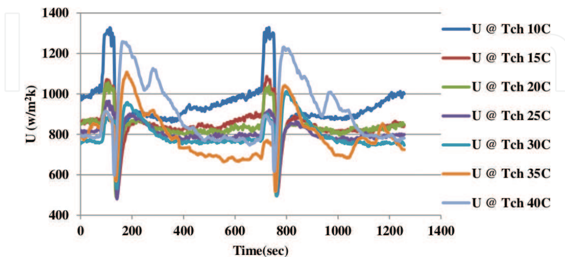
Figure 8. Typical experimental overall heat transfer coefficient profiles at 60000 ppm salt concentration.
