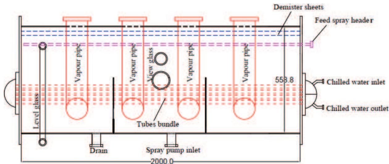
Figure 3. Adsorption desalination cycle evaporator detailed design.
