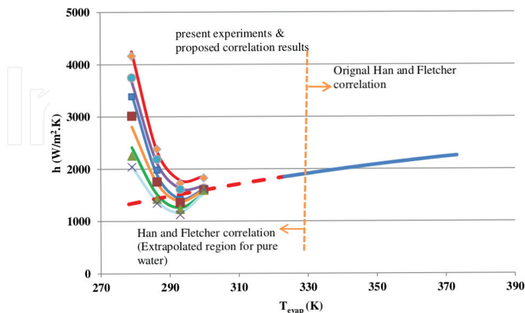
Figure 12. Falling film heat transfer coefficient values: experimental and proposed correlation compared with Han and Fletcher correlation extrapolated region.
