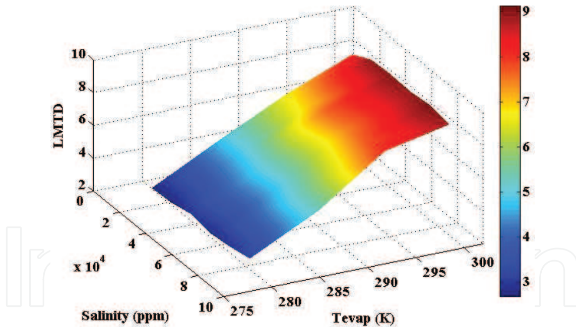
Figure 14. Effect of evaporator saturation temperature and feed salt concentration on LMTD.
