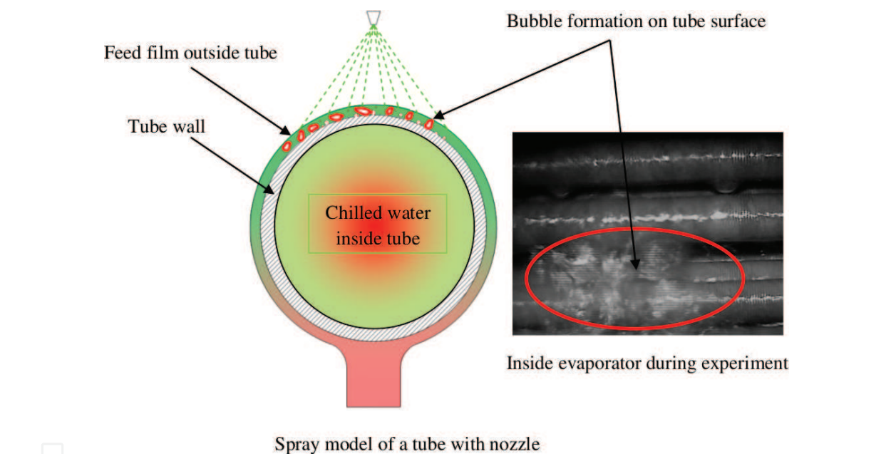
Figure 5. Bubbles formation in liquid film on tube surfaces and film agitation effect captured by camera.
