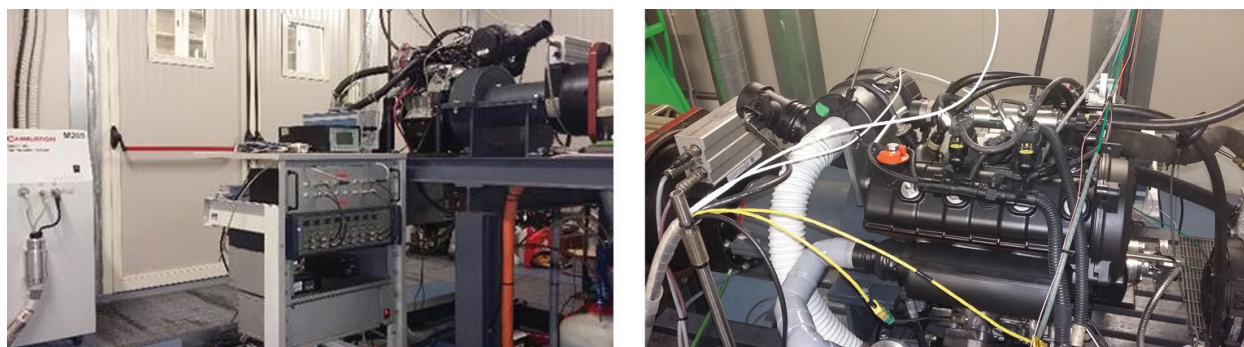
Figure 1. Engine setup.
