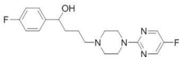
BMY 14802 ( 22 ); pIC_{50} 5-HT 1A = 6.7
