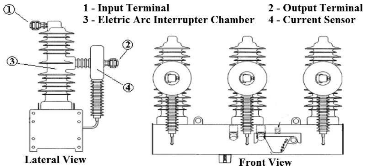
Figure 2. Recloser.
