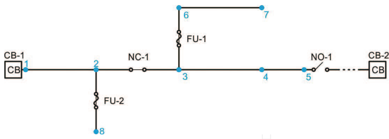
Figure 4. Example distribution network.
