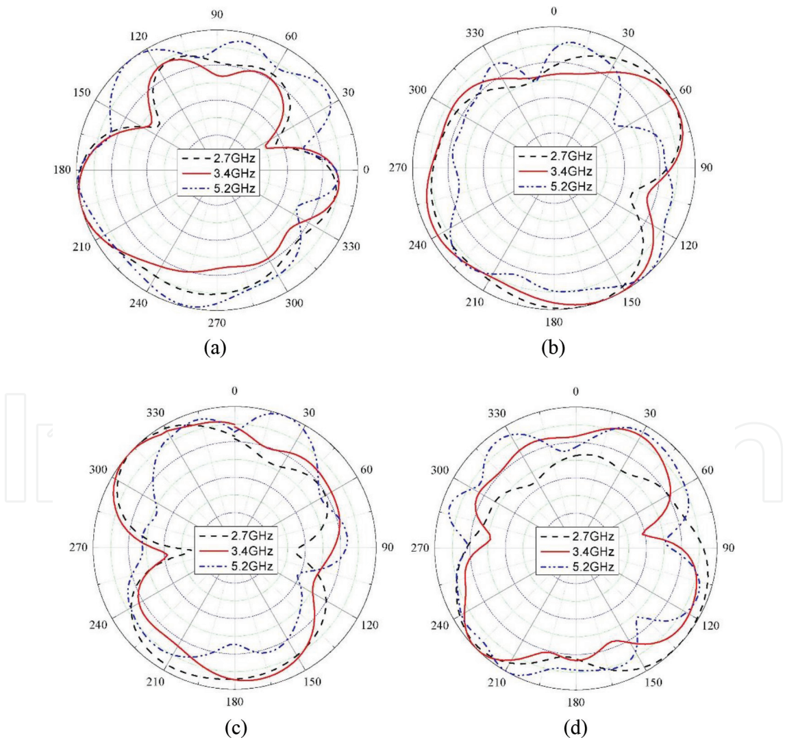
Figure 21. Radiation patterns of the CR-UWB antenna. (a) E-plane of mode 4. (b) H-plane of mode 4. (c) E-plane of mode 5. (d) H-plane of mode 5.
