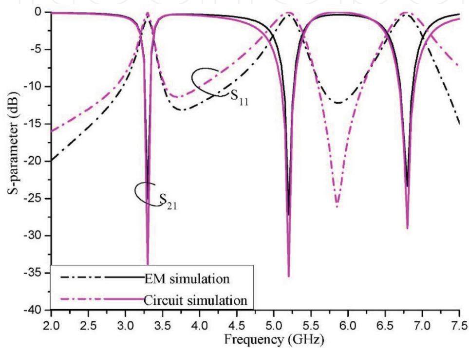
Figure 15. Comparisons of the tri-band stop-band filter.
