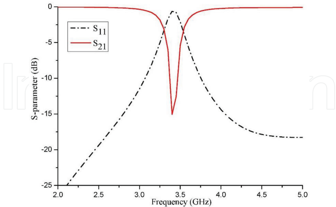
Figure 3. Performance of the DMS band-stop filter.
