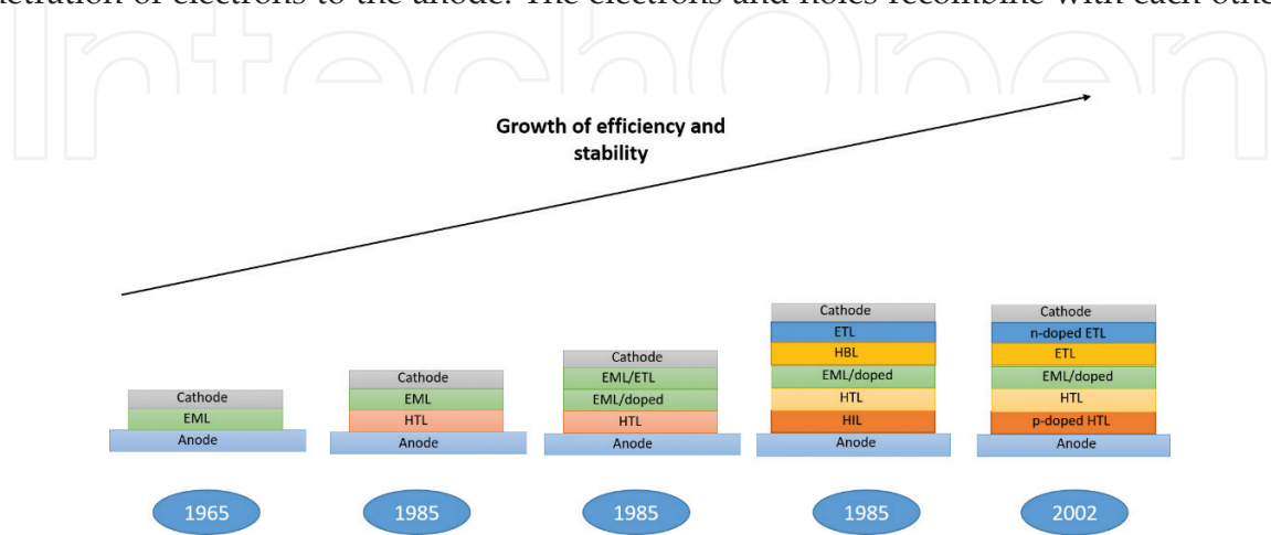
Figure 3. Evolution of OLED device structure.
