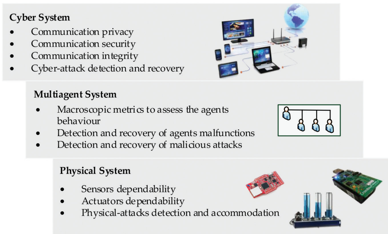
Figure 4. Agent features.
