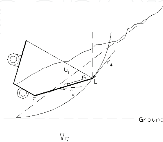
Fig. 5. Medium force components on a bucket
