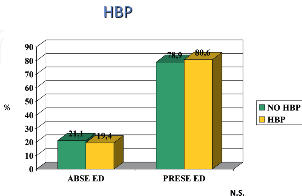
Graph 4. HBP%. N.S.
