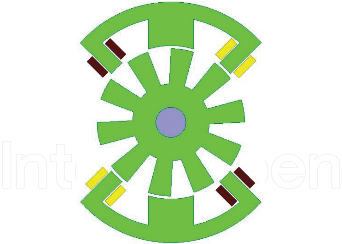
Figure 14. A common pole E-core SRM configuration.
