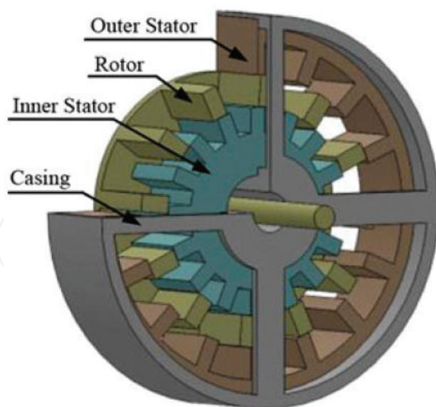
Figure 28. Primary 3-D model of designed DSSCR-SRM.
