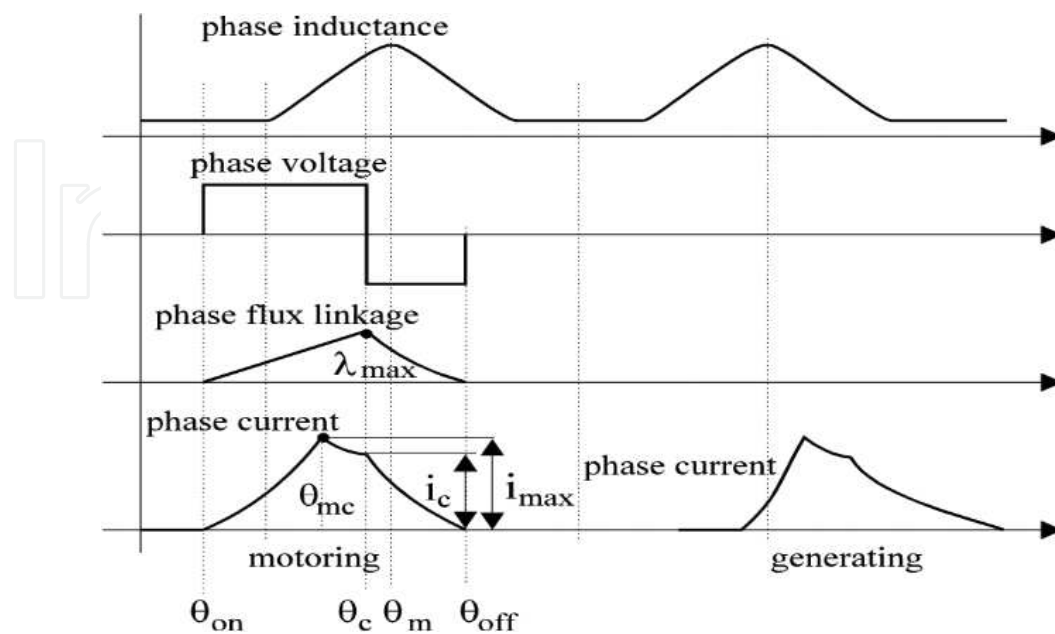
Figure 6. Phase inductance, phase voltage, phase flux linkage and phase current.
