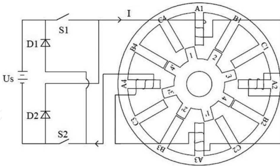
Figure 9. A 12:8 pole three-phase SRM generator configuration.
