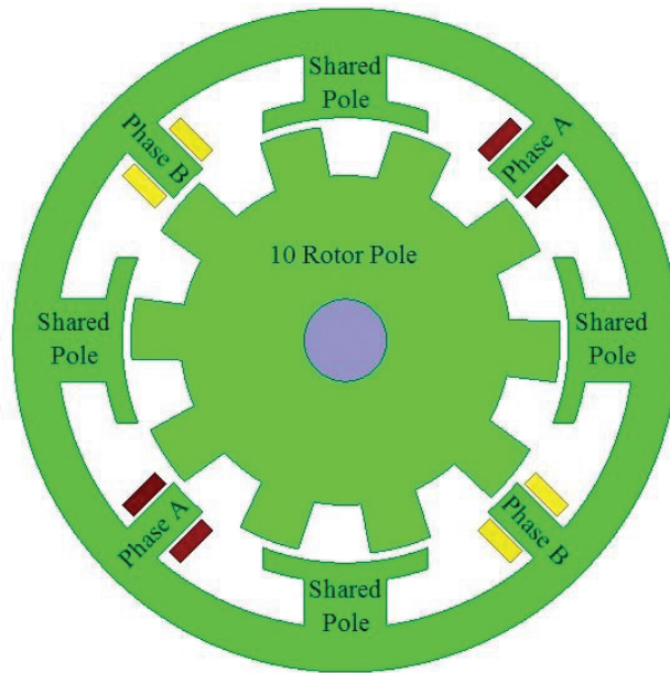
Figure 16. A common pole E-core SRM configuration.
