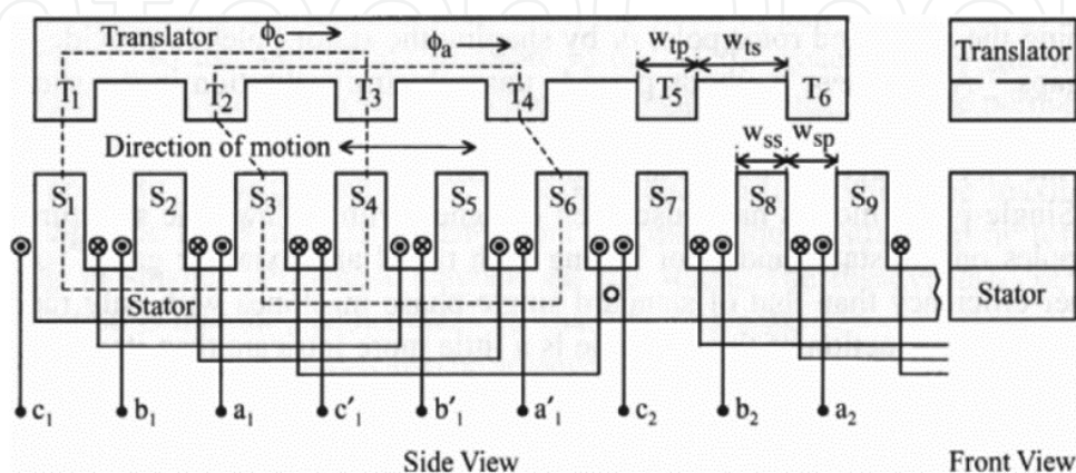
Figure 11. LSRM structure.
