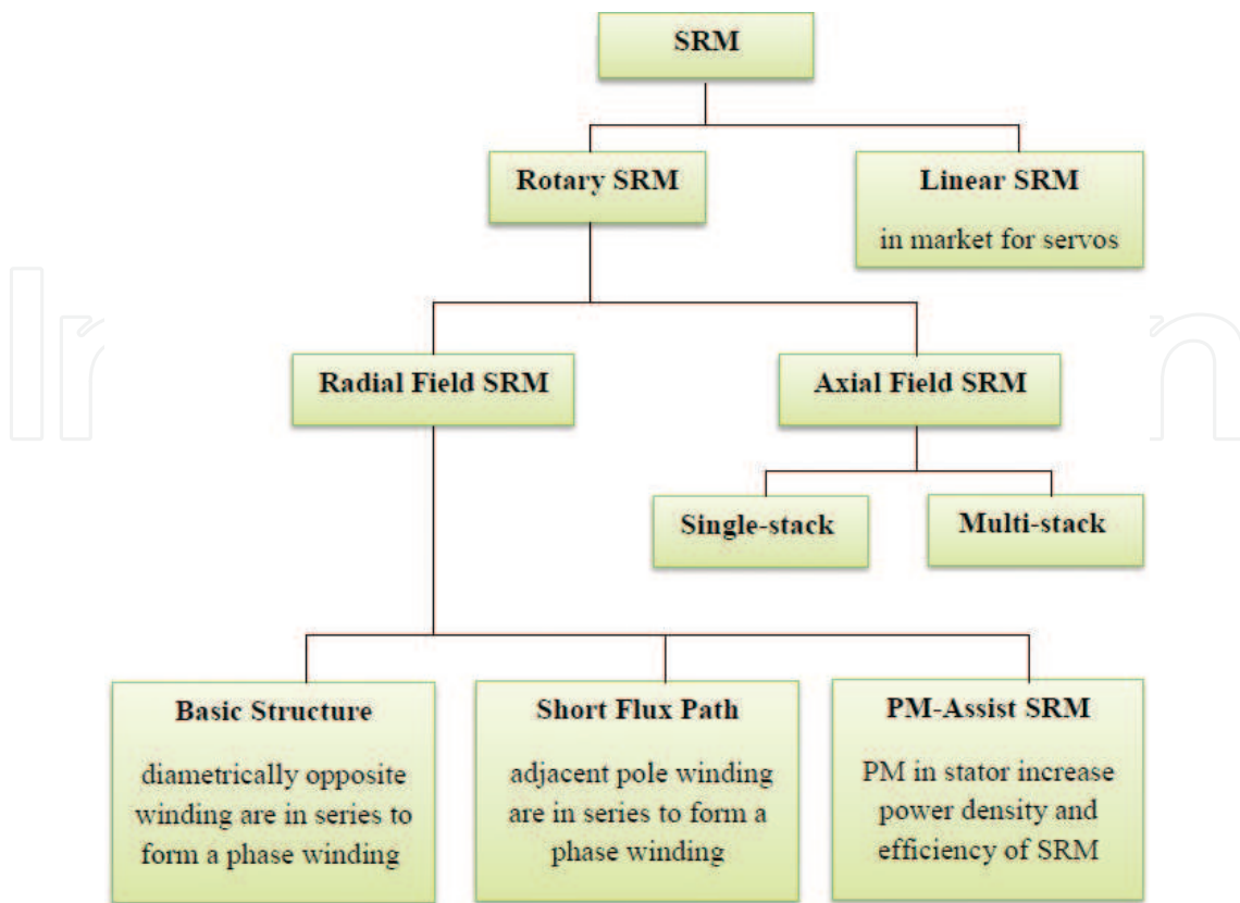
Figure 2. SRM classification based on movement pattern, flux path, and type of excitation.
