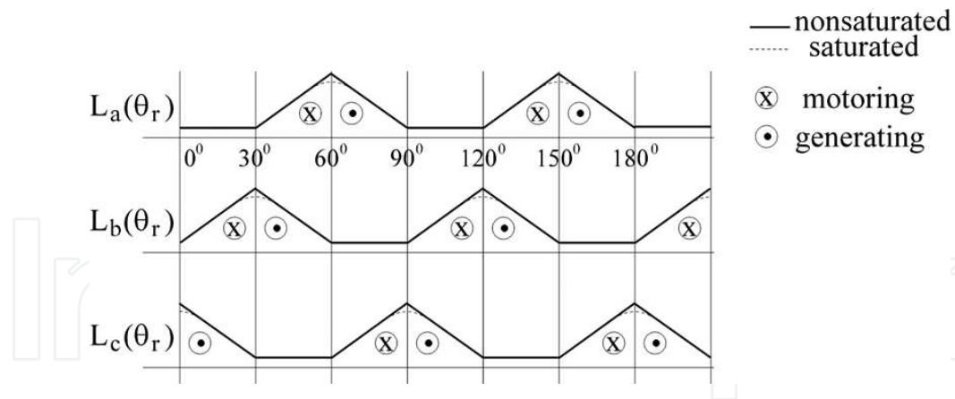
Figure 4. Phase inductance and operation modes in a 4:6 SRM.
