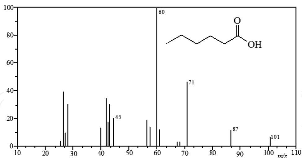
Figure 18. Hexanoic acid-simplified mass spectrum [1].
