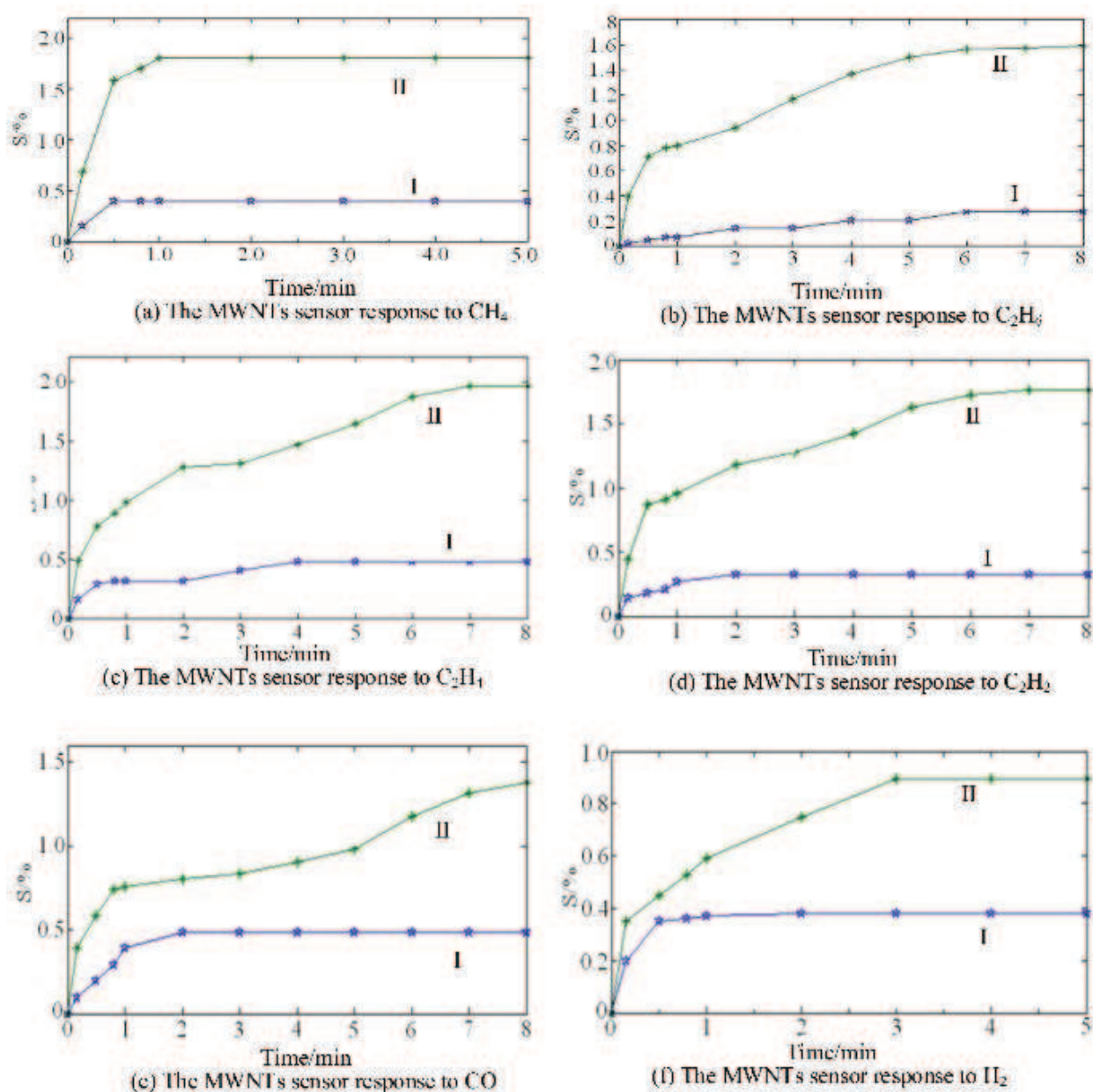
Figure 11. The MWNTs sensor response to \text{CH}_4 , \text{C}_2\text{H}_6 , \text{C}_2\text{H}_4 , \text{C}_2\text{H}_2 , CO, \text{H}_2 .
