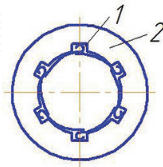
Figure 1. Aerodynamic bearing: 1—trunnion; 2—foil.
