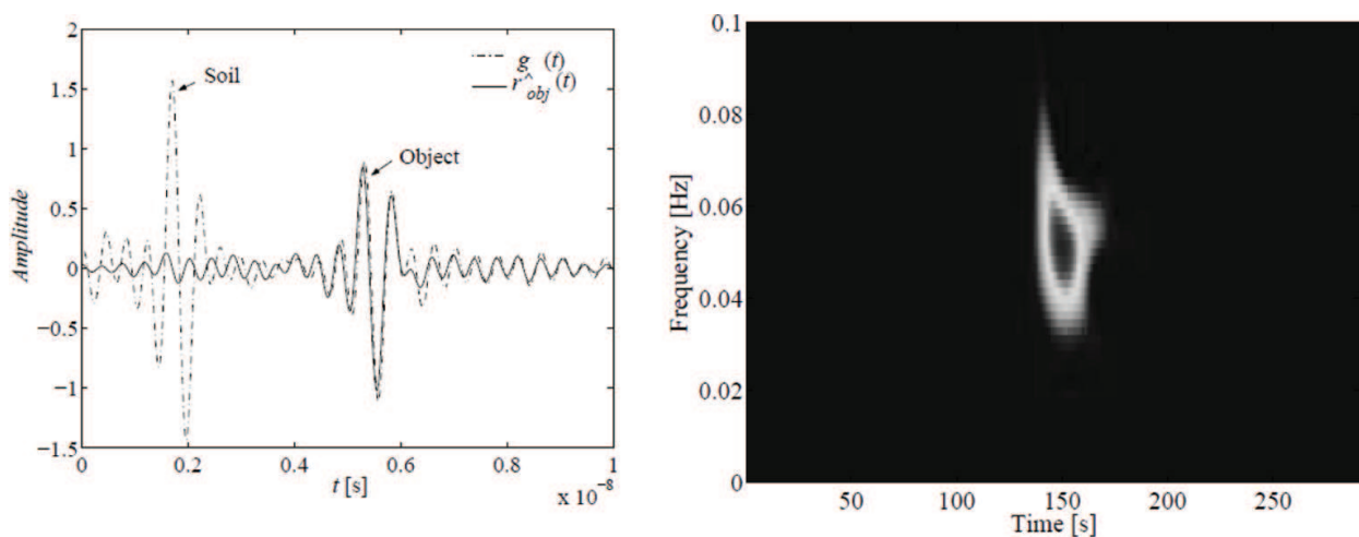
Figure 23. WVD (right) applied to a filtered and migrated A-scan data (left) for an antitank landmine buried in sand (from Figure 16 ).
