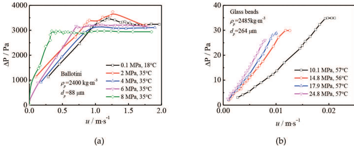
Figure 2. Bed pressure drop vs. superficial velocity for SCCO 2 fluidized bed: (a) Marzocchella and Salatino [11], and (b) Vogt et al. [12].
