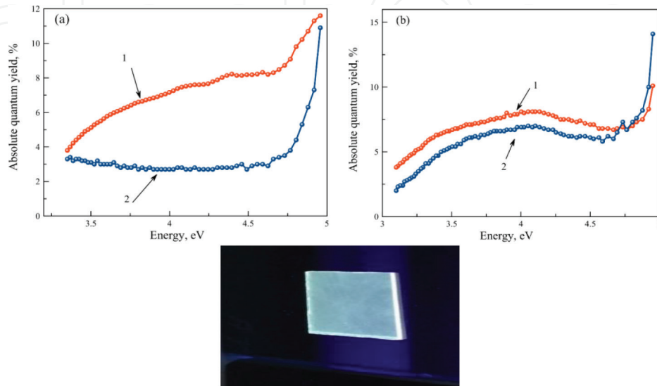
Figure 16. (a) Absolute quantum yield for the glasses doped with PbS as-prepared (1) and glass after heat treatment (2), (b) Absolute quantum yield for glass doped with PbSe as-prepared (1) and after heat treatment (2) and (c) photography of the (\text{PbS})_n MCs luminescence at \lambda_{\text{exc}} = 365 nm.
