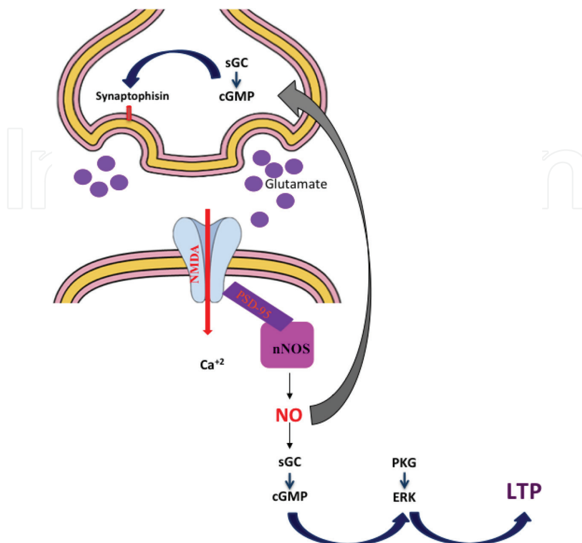
Figure 1. NO act as an unconventional neurotransmitter that is not stored in synaptic vesicles and not released upon membrane depolarization; it releases as soon it is synthesized and does not bind to any receptors, but diffuses from one neuron to another. NO stimulate soluble guanylyl-cyclase to form the second messenger molecule, cyclic guanosine monophosphate (cGMP) either as a post- or a presynaptic messenger. PKG, protein kinase G; ERK, extracellular signal-regulated kinases; LTP, long-term potentiation. Images: https://mindthegraph.com .
