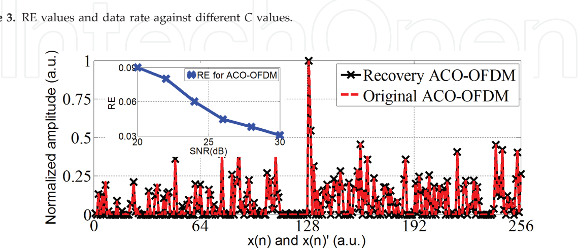
Figure 3. RE analysis for ACO-OFDM (with N = 256 ) for SNR of 30 dB. The inset shows the RE for 20 < \text{SNR} < 30 dB.
