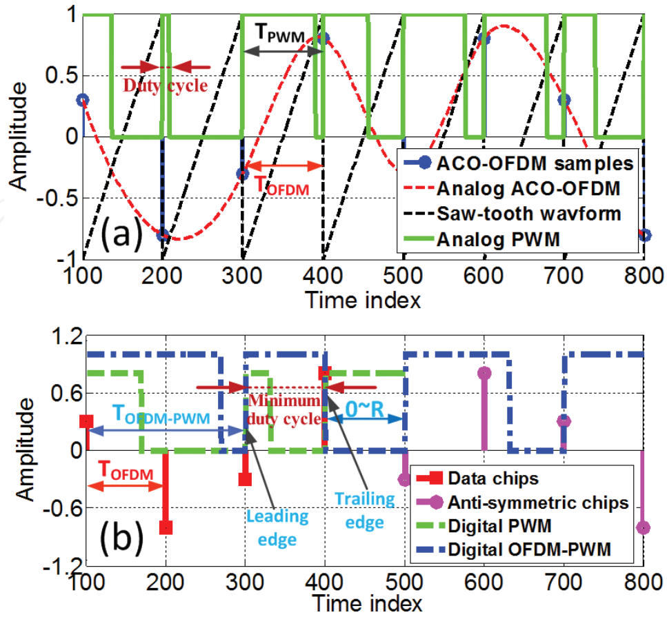
Figure 6. Time-domain waveforms for (a) ACO-OFDM, ramp, and PWM and (b) the process of the digital OFDM-PWM generation.
